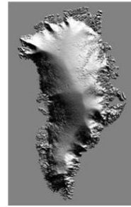
Figure 2. Greenland DEM Data Set
