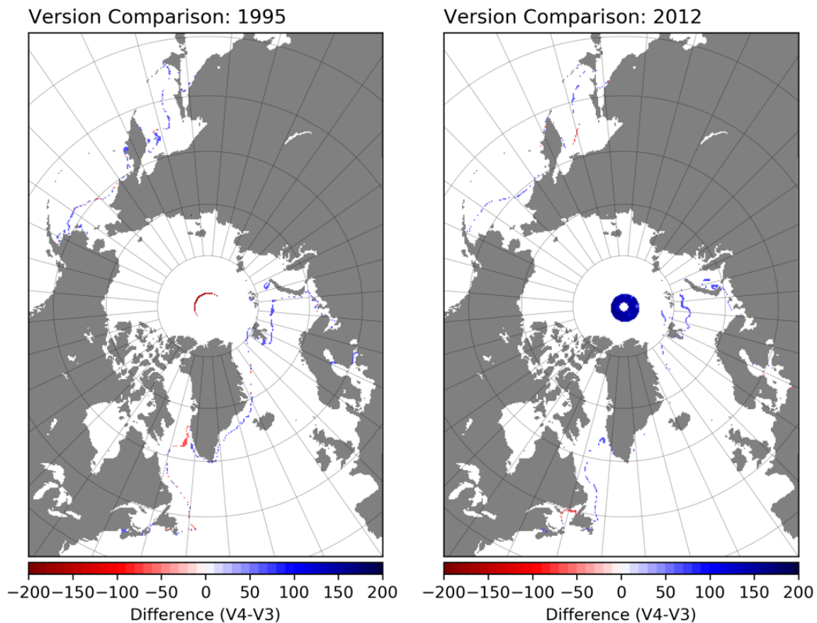
Figure 3. Visual comparison of snow melt onset dates from Version 3 and Version 4 of this data set.
