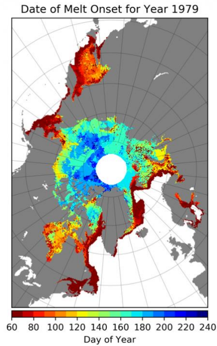
Figure 1. Sample browse image showing snow melt onset dates for 1979.
