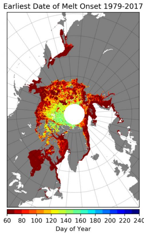
Figure 2. Sample statistical-field browse image showing the earliest snowmelt onset date recorded between 1979 and 2017.
