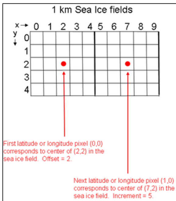
Figure 3. This figure shows how MOD29/MYD29 1 km data fields map to 5 km latitude and longitude geolocation fields.
