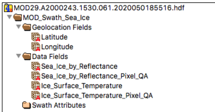
Figure 2. This figure shows the MYD29 fields included in each data file as displayed with HDFView software.
