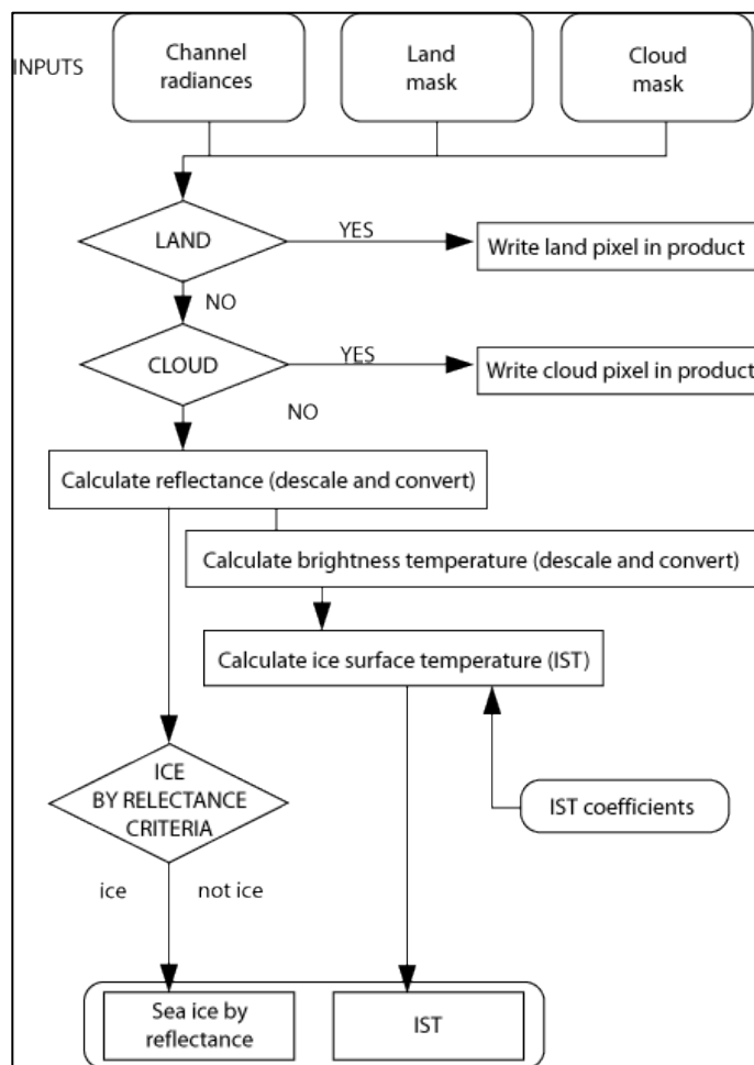
Figure 4. Flowchart showing the MOD29 and MYD29 sea ice algorithm
