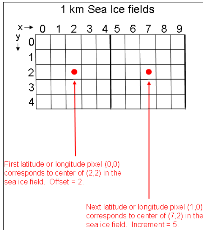
Figure 1. Offset and increment for MODIS 1 km swath data.
