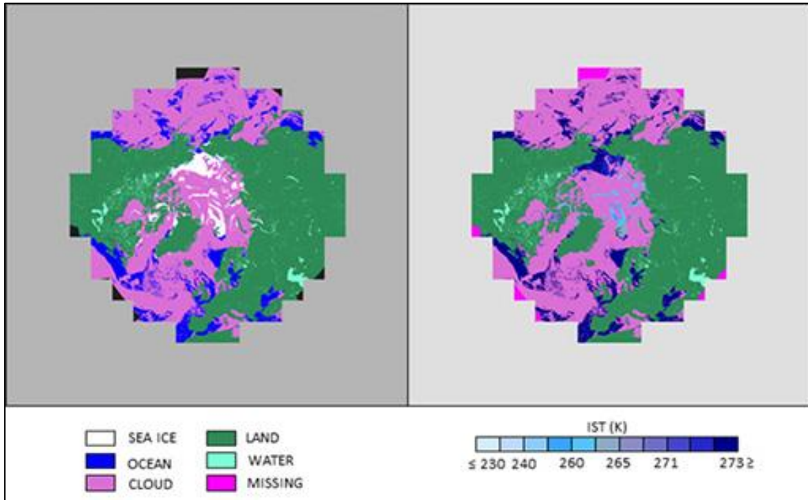
Figure 1. Typical MODIS 4 km daily Northern Hemisphere sea ice extent (left) and IST (right) data.
