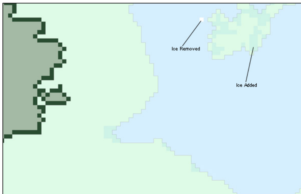
Figure 8. Illustration of Closing Operation: The medium green on the left side is land; the dark green surrounding it is coastline. The area of the lightest green is the sea ice area prior to the closing operation. The light green within the lightest green is sea ice added during the closing operation. The single stand-alone white cell was marked as sea ice in the input IMS product, but is eliminated when sea ice polygons smaller than 16 cells, or roughly 256 sq km, are discarded. The grey line around the light and lightest green is the smoothed ice edge.
