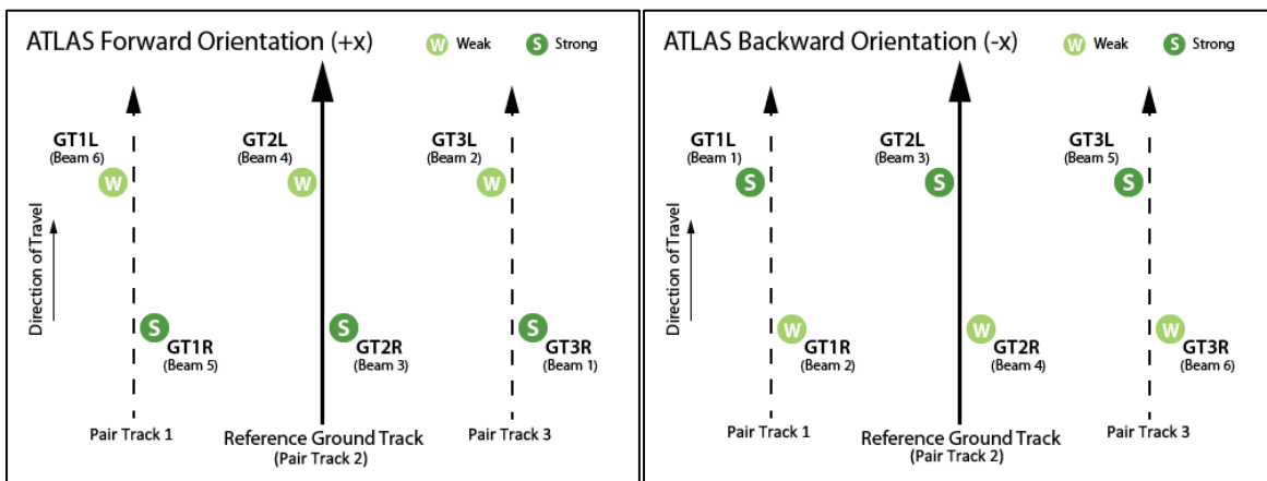
Figure 1. Spot and ground track (GT) naming convention with ATLAS oriented in the forward (instrument coordinate +x) direction.
