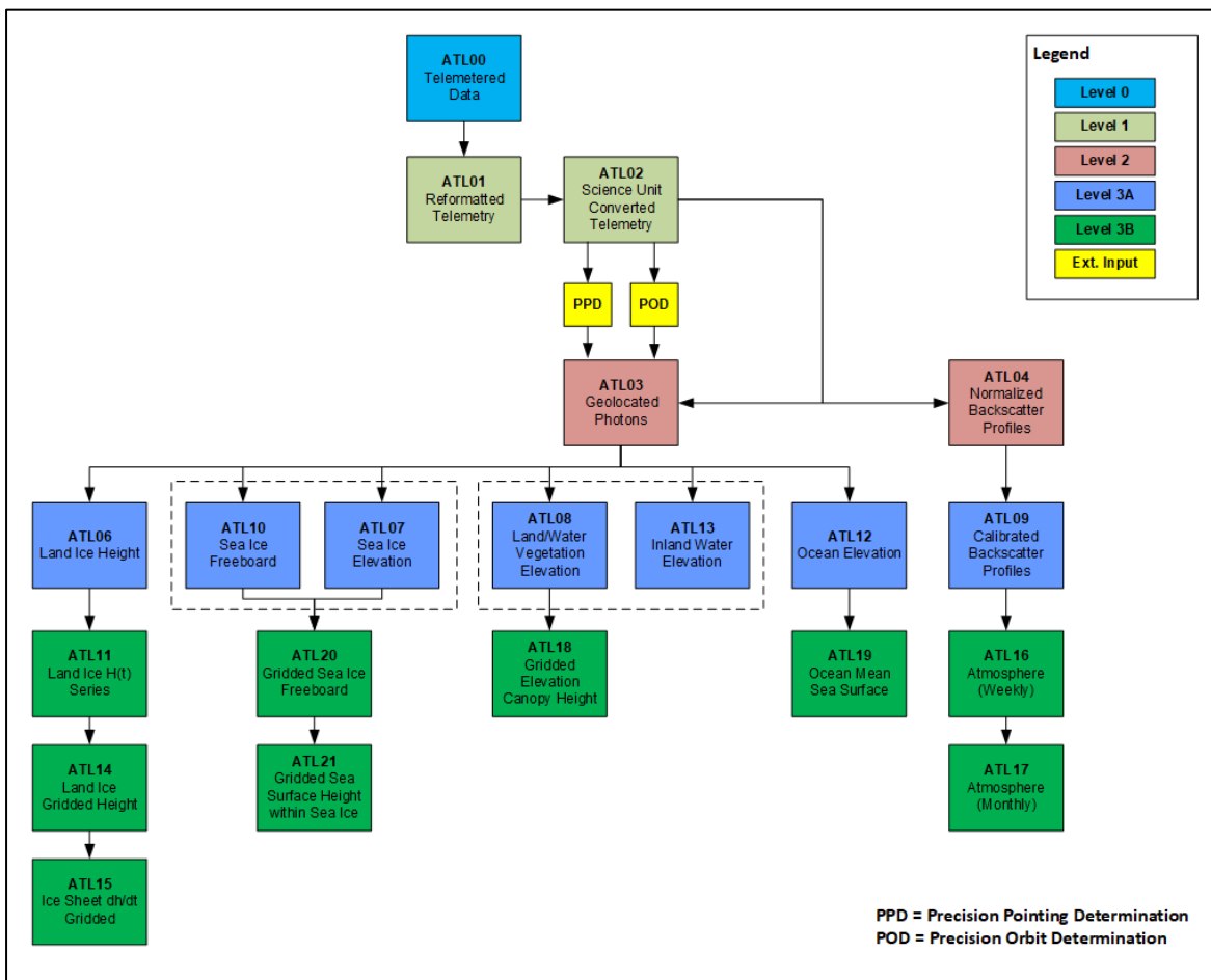
Figure 5. ICESat-2 data processing flow. ATL02 processing converts ATL01 data to science units and applies instrument corrections. The Precision Pointing Determination (PPD) and Precision Orbit Determination (POD) solutions compute the pointing vector and position of the ICESat-2 observatory.
