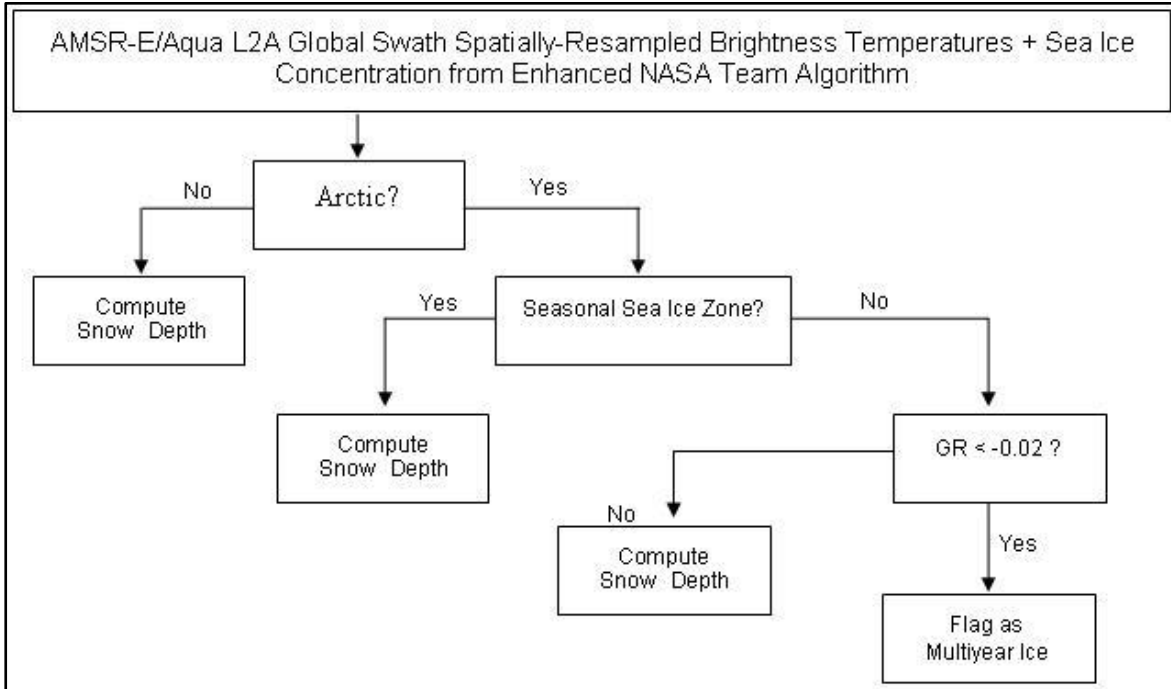
Figure 4. Processing Sequence for AMSR-E 25 km Sea Ice Products
