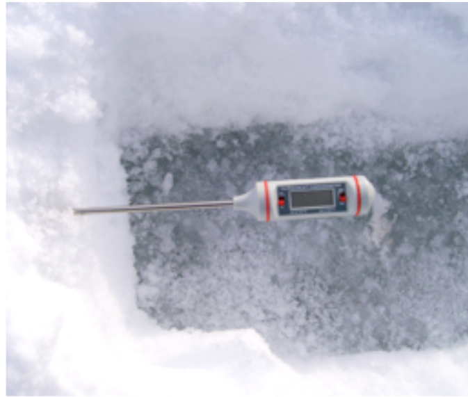
Above left: A digital thermometer inserted into a hole at a 45-degree angle to measure surface sea ice temperature (Section 4.3 and Figure 12). Above right: A digital thermometer inserted horizontally into the snow 5 cm from the ice surface (Section 4.4 and Figure 12). Photos: Nina Palituq
