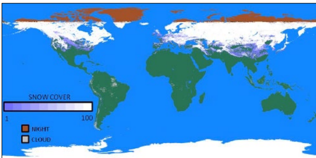
Figure 1. This figure shows MOD10CM (MODIS/Terra) monthly mean snow cover mapped to a CMG, for January 2003.
