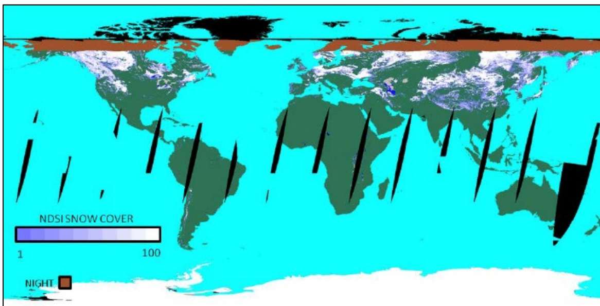
Figure 1. This MOD10C1 snow map shows the percent of snow cover mapped to a 0.05° CMG (approx. 5 km). The data was acquired 9 January 2003 from MODIS/Terra, but provides a representative sample of the same data acquired from MODIS/Aqua.
