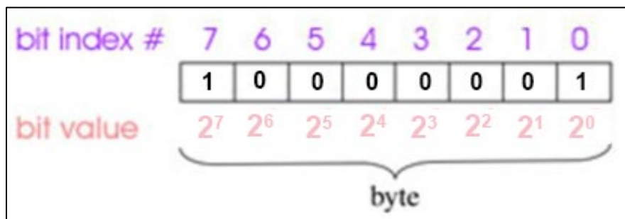
Figure 2. This figure shows the decoded bit flag for the 8-bit integer value 129. Bit positions are numbered from right (bit 0) to left (bit 7), and each bit stores the result of a screen. In this example, bit 0 (inland water) and bit 7 (low illumination) are set to true (1).
