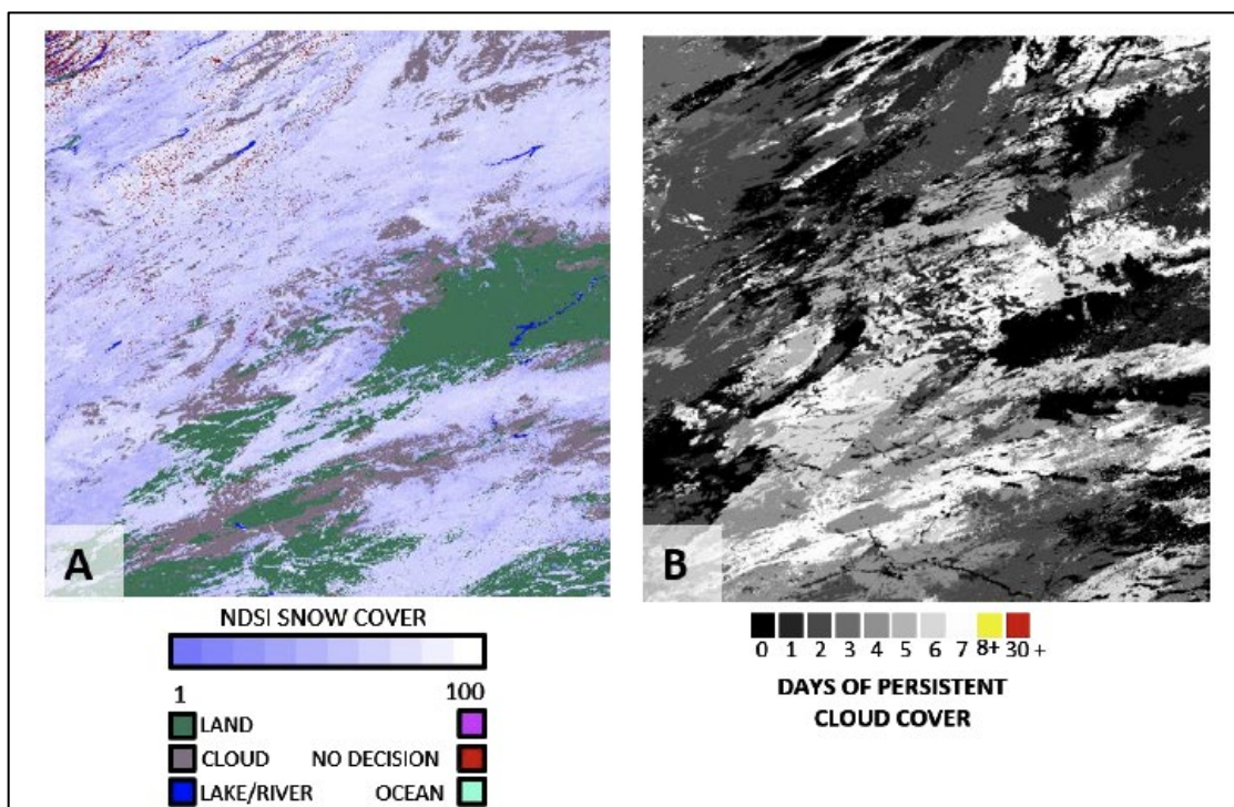
Figure 4. This figure shows CGF_NDSI_Snow_Cover (A) and cloud persistence (B) from MOD10A1F, tile h10v04, (26 December 2017, MODIS/Terra). The region shown extends from southern Nebraska to northern Montana. The unlabeled purple square in the legend represents 'Night'.
