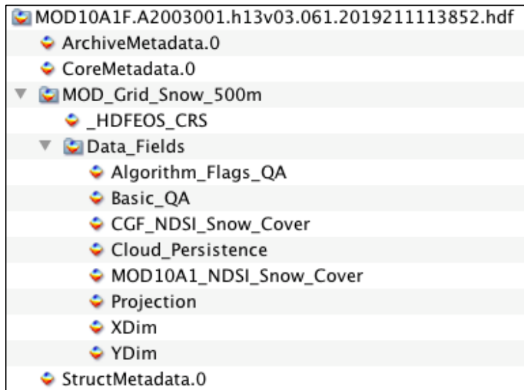
Figure 1. This figure shows the fields included in each MYD10A1F data file as displayed with Panoply software.
