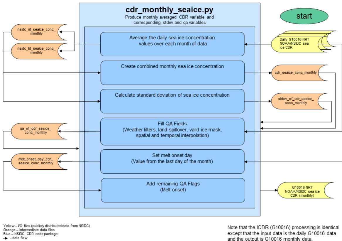
Figure 2. Flow of Data through the Monthly NRT CDR Processing.
