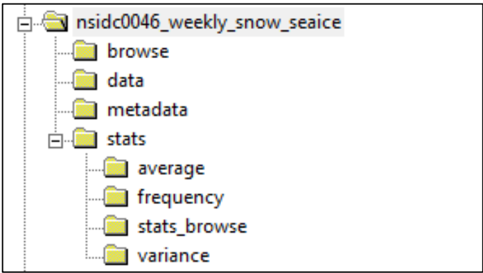
Figure 2. Directory Structure.
