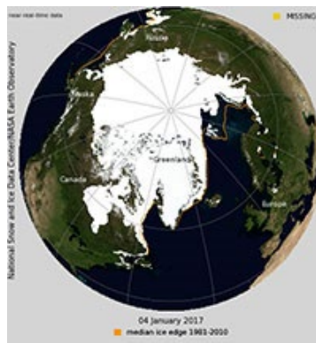
Figure 13c. Blue Marble Daily Sea Ice Extent Image for the Northern Hemisphere.
