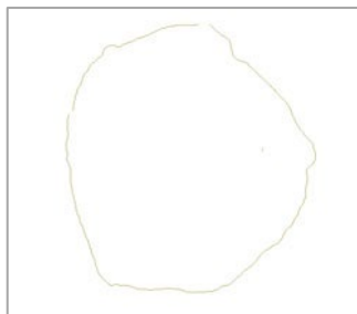
Figure 11b. Southern Hemisphere Median Shapefile for month of April, 1981 - 2010.
