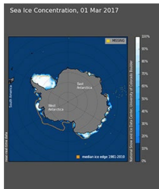
Figure 12b. Daily Sea Ice Concentration Image for the Southern Hemisphere.
