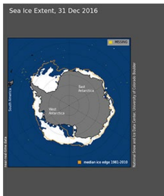
Figure 13b. Daily Sea Ice Extent Image for the Southern Hemisphere.
