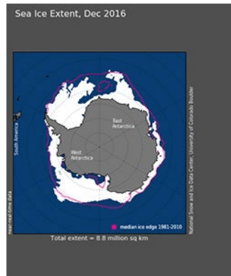
Figure 5b. Monthly Sea Ice Extent Image for the Southern Hemisphere.
