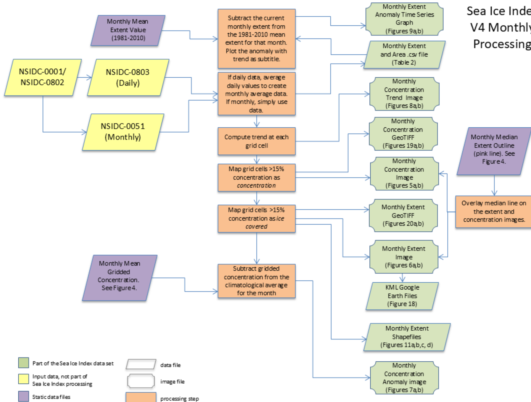
Figure 24. Sea Ice Index Monthly Product Processing Using GSFC Product
