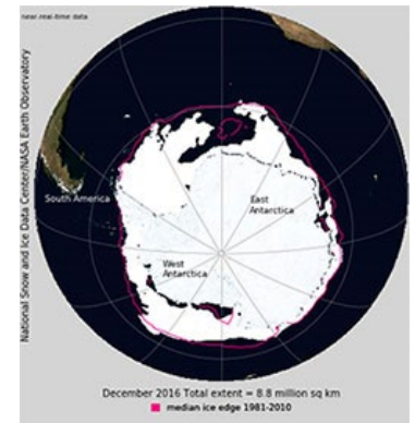
Figure 5d. Blue Marble Version of the Monthly Sea Ice Extent Image for the Southern Hemisphere.
