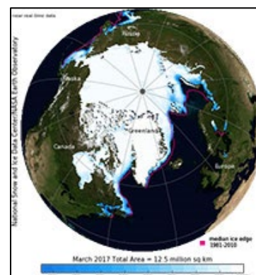
Figure 4c. Blue Marble Version of the Monthly Sea Ice Concentration Image for the Northern Hemisphere.
