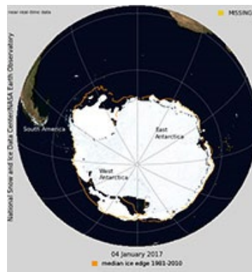
Figure 13d. Blue Marble Daily Sea Ice Extent Image for the Southern Hemisphere.
