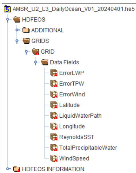
Figure 1. HDF-EOS5 Internal Structure as seen in HDFView
