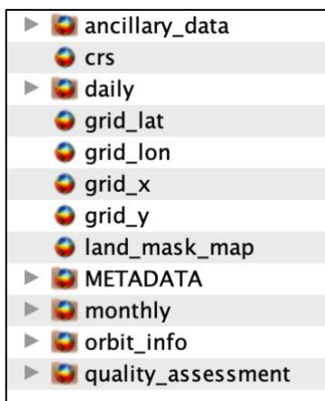
Figure 1. ATL20 top-level data groups and variables.
