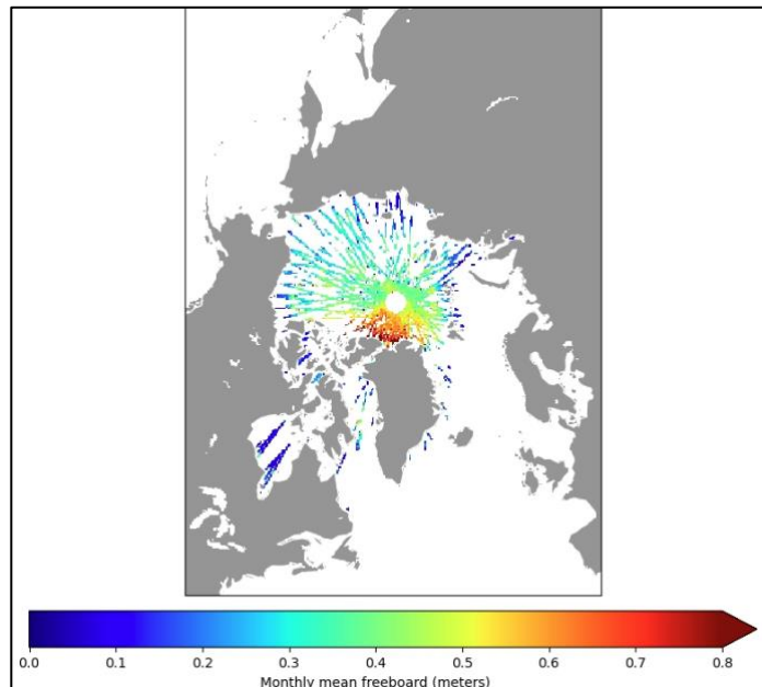
Figure 2. Example browse image of monthly mean freeboard ( mean_fb ).
