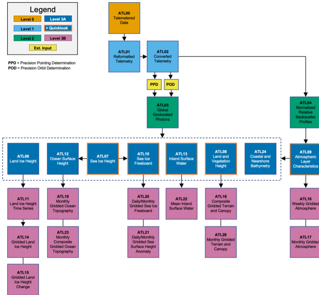
Figure A - 2. Schematic of ICESat-2 data processing and data products.
