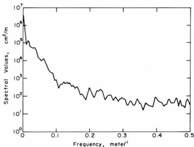
Figure 12. Power spectral density curve for multiyear ice.
