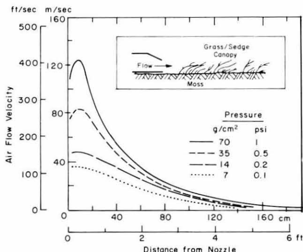
Figure 27. Dissipation of horizontal air flow velocity through tundra plant canopy.
