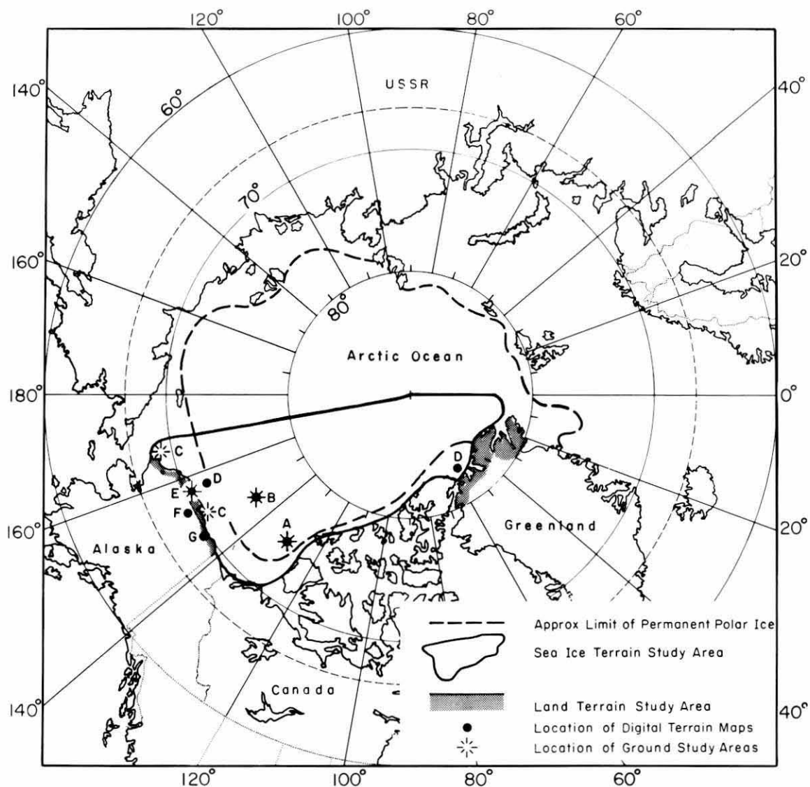
Figure 5. Sea ice and terrestrial surface geometry study areas.
