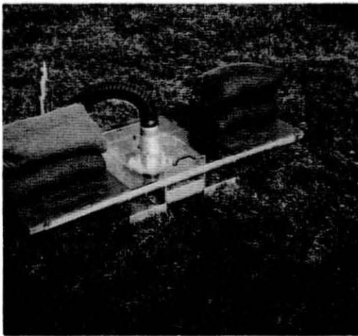
a. Cushion pressure simulation box.
