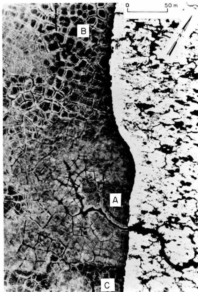
Figure 17. Airphoto taken in the Barrow area showing the range of polygon types commonly found on the coastal plain. A: little apparent relief. B: low-centered polygons. C: high-centered polygons.
