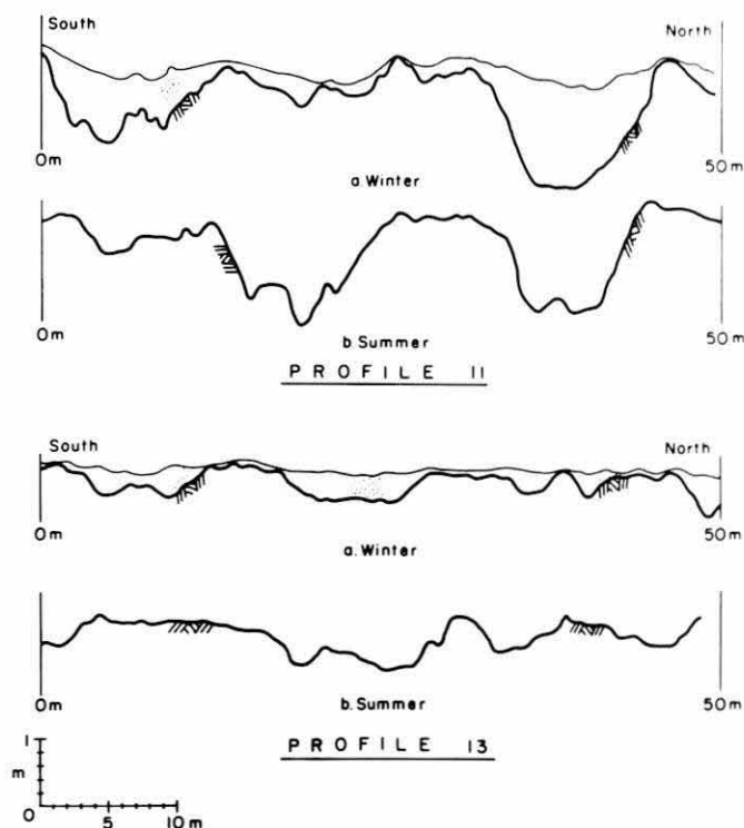
Figure 18. Winter and summer land profiles from the Barrow area indicating subduing of microrelief by snow cover.
