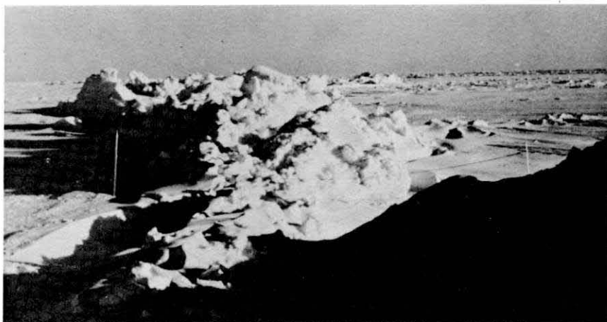
Figure 3. First-year ridge about 5 ft (1.5 m) high in the Beaufort Sea.
