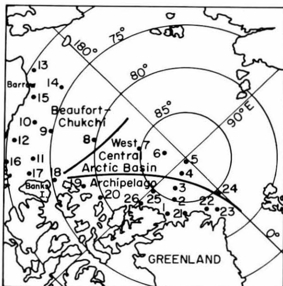
Figure 10. Geographical sampling regions for laser data.
