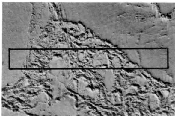
Figure 6. Digital terrain map of polygonal ground in the Barrow area.
