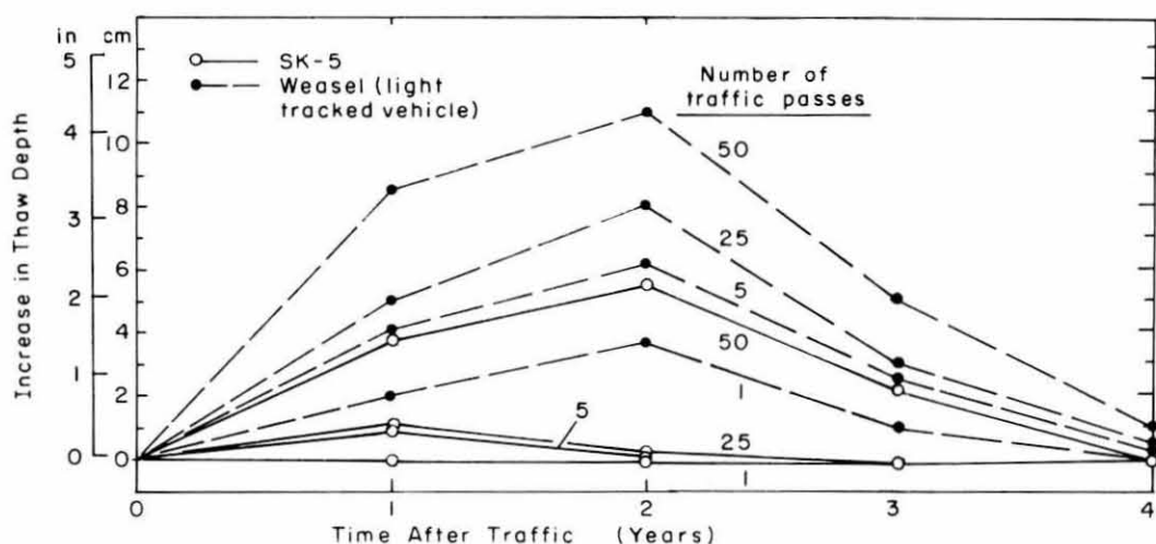
Figure 24. Effect of SK-5 and Weasel traffic on the thaw depth of wet meadow tundra.
