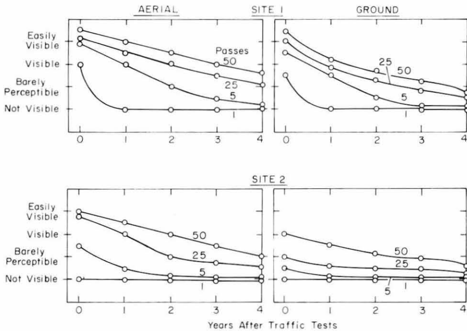
Figure 23. Relative visibility of SK-5 traffic signatures.
