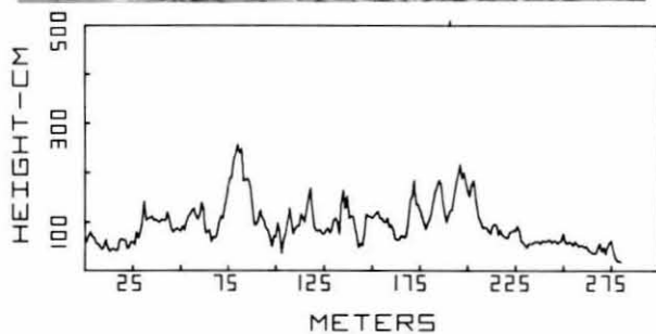
Figure 8. Digital terrain map of first-year ice with hummocks and brash ice.
