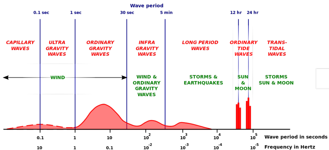
Figure 2-1 Classification of water wave types after Munk (1950).
