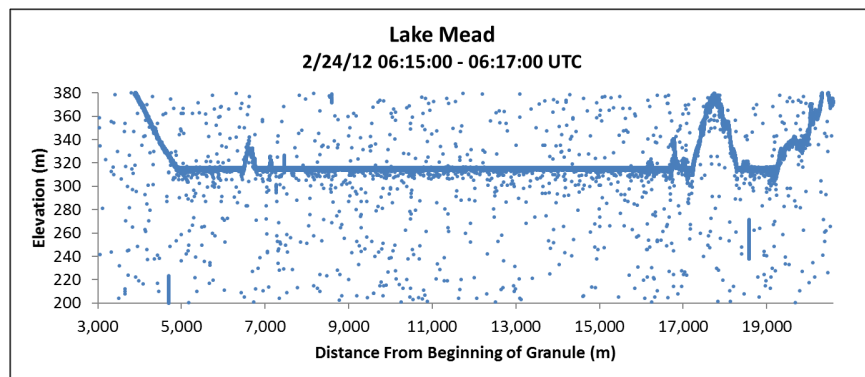
Figure 2-9 Photon cloud data from 2012 MABEL flight over Lake Mead (Jasinski et al., 2016).
