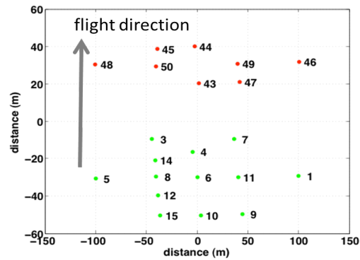
Figure 2-8 Configuration of MABEL beams.
