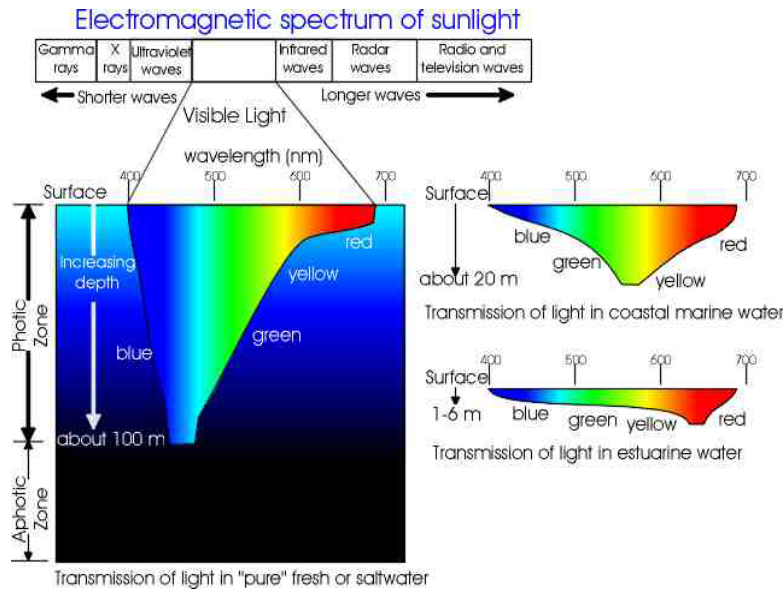
Figure 2-5 Comparative representation of light penetration in natural water including open ocean (left), coastal marine (top right) and estuary (bottom right). (from Buchheim, Oceanography http://www.marinebiology.org/oceanography.htm )
