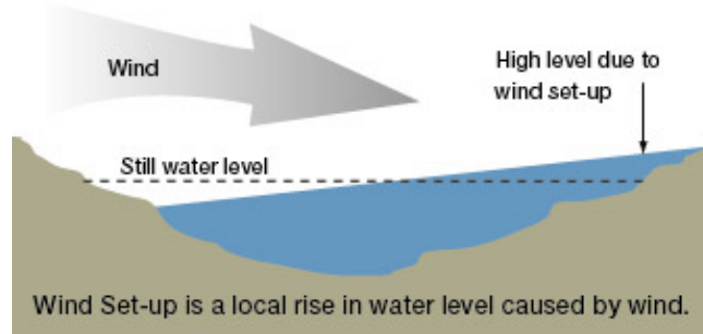
Figure 2-4 Representation of wind set-up due to prevailing winds (graphic from http://www.seagrant.umn.edu/superior/processes ).
