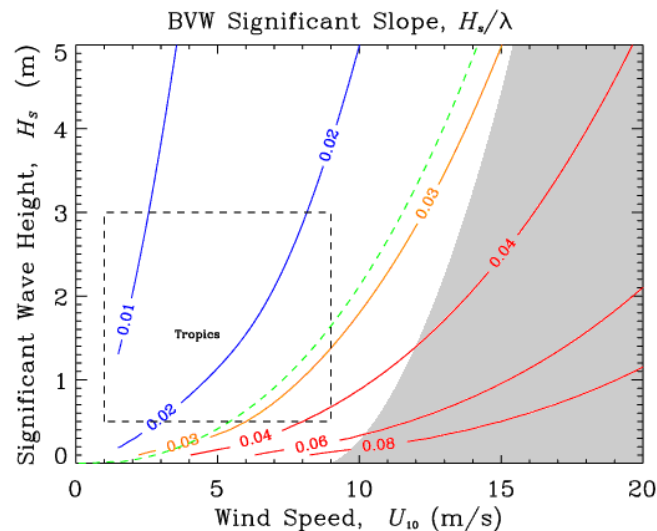
Figure 2-3 Relation among significant wave height, H_s , significant wave slope, H_s/\lambda where \lambda is dominant wavelength, and wind speed U_{10} . Green line shows local-equilibrium values predicted by Bourassa et al. (1996) Blue and red lines represent falling (swells) and rising seas, respectively. (From http://coaps.fsu.edu/papers/use_significant_derived_stress/ ).
