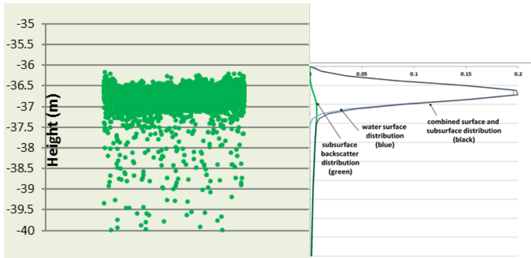
Figure 3-2 ATL13 Water Model: Conceptual interpretation of ATLAS photon cloud histogram over inland waters consisting of integrated surface reflected and subsurface volume scattered photons.
