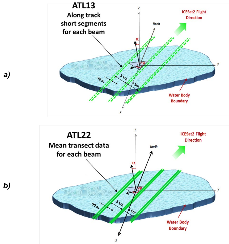
Figure 1-2 a) Schematic of principal ATL13 Inland Surface Water along track short segment data products for each weak and strong beam. Products include surface height statistics, subsurface attenuation, significant wave height (SWH) and coarse bottom topography. Height statistics are reported for variable segment lengths of 100 signal photons. Estimated accuracy is 5-8 cm per 100 signal photons. b) Comparison schematic of principal ATL22 Release 4 Mean Inland Surface Water data products computed for each weak and strong beam crossing.
