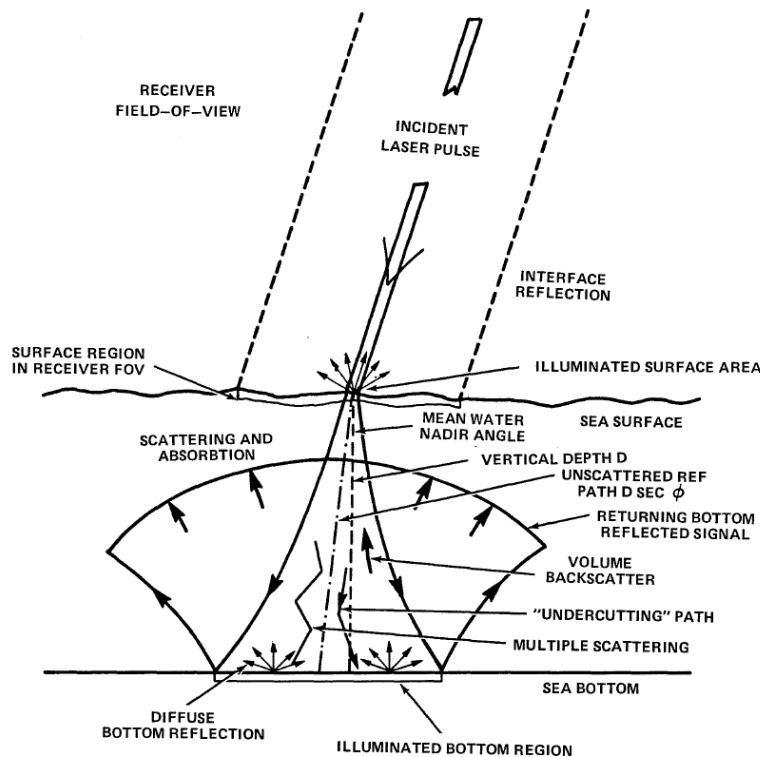
Figure 2-6 Sketch of process lidar subsurface backscattering processes in shallow water (from Guenther, 2000)
