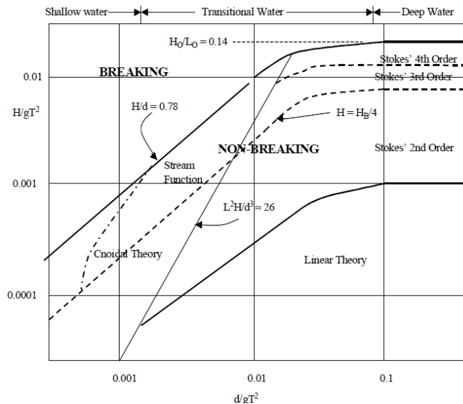
Figure 2-2 Parameter space for wave theories based on normalized height ( H/gT^2 ) and water depth ( d/gT^2 ) where g is gravity constant and T is wave period, after Le Mehaute (1976).
