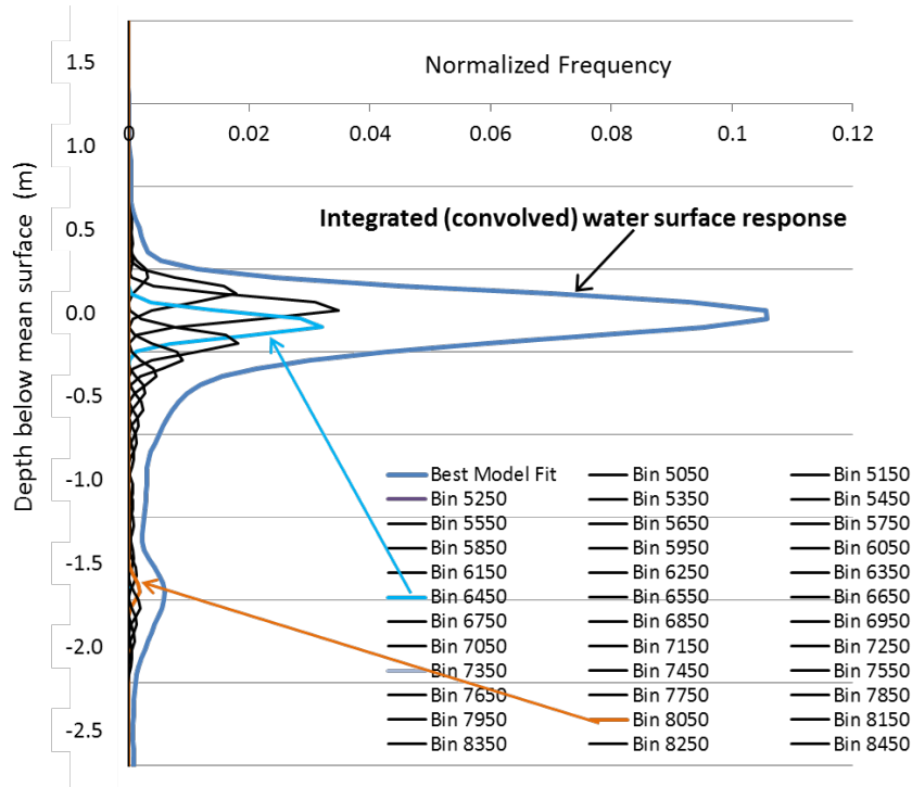
Figure 4-7 Constrained Deconvolution Method – Integrated response to all MABEL bins.
