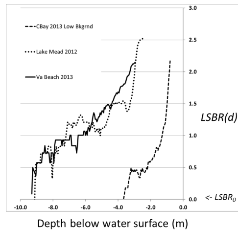
Figure 6-3 Signal to background ratio profiles versus depth, LSBR(d) , for cases presented in this study, expressed in \log_{10} base. Also indicated is the LSBR_0 threshold level. (Jasinski et al., 2016).
