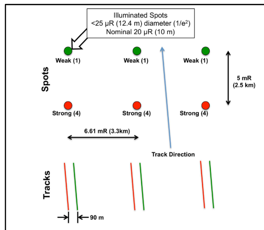
Figure 1-1 ICESat-2 ATLAS six-beam configuration.
