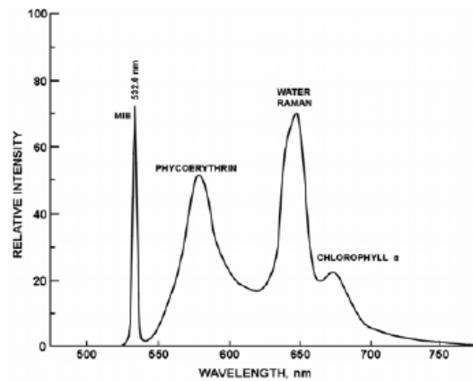
Figure 2-7 Backscattered spectra from natural water sample excited at 532 nm (based on Exton et al., 1983, and Pe’eri et al, 2007).
