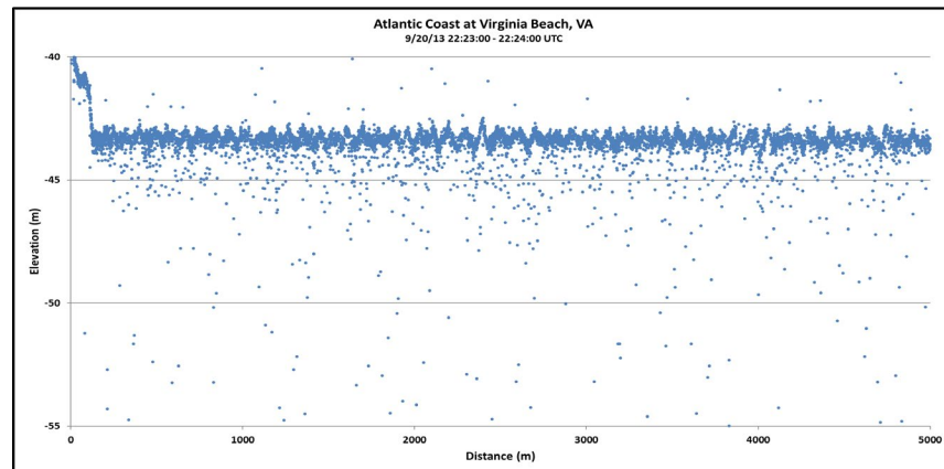
Figure 2-10 Photon cloud data from 2013 MABEL flight over Atlantic Coast near Virginia Beach identifies surface waves and beam attenuation (Jasinski et al., 2016).
