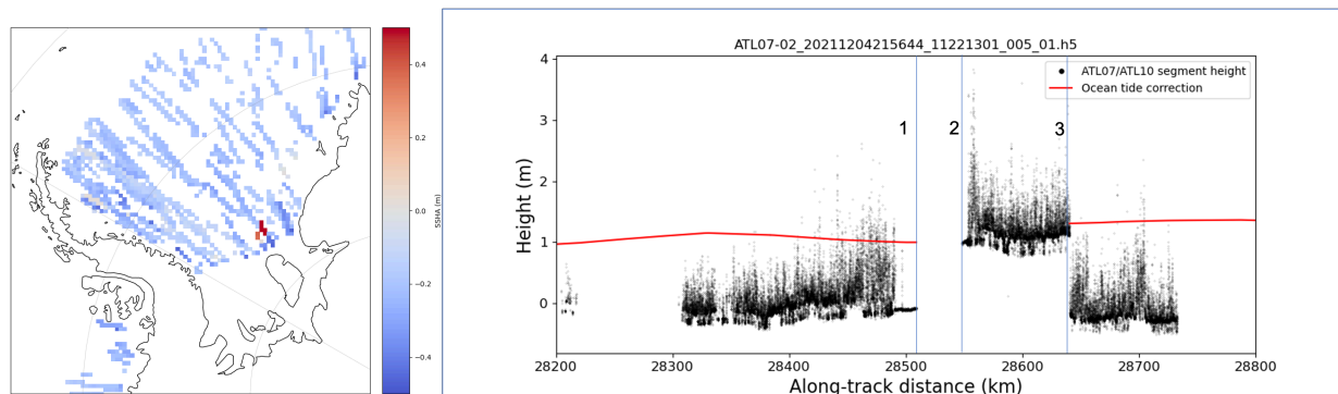
Figure 8: (left) gridded composite of ATL10 Sea Surface Height Anomalies (SSHA) from Dec 1-22, 2021, (right) ATL07 heights (black markers) for a granule extending over the Weddell Sea (over the positive SSHA shown on the left). ATL07 is missing between vertical lines 1 and 2 due to the presence of an iceberg and the effect of the coarse height filter (confirmed by ATL03) while the ocean tides (~1 m, red line) are missing between lines 1 and 3 resulting in the unphysical step-change in ATL07 between lines 2 and 3.
