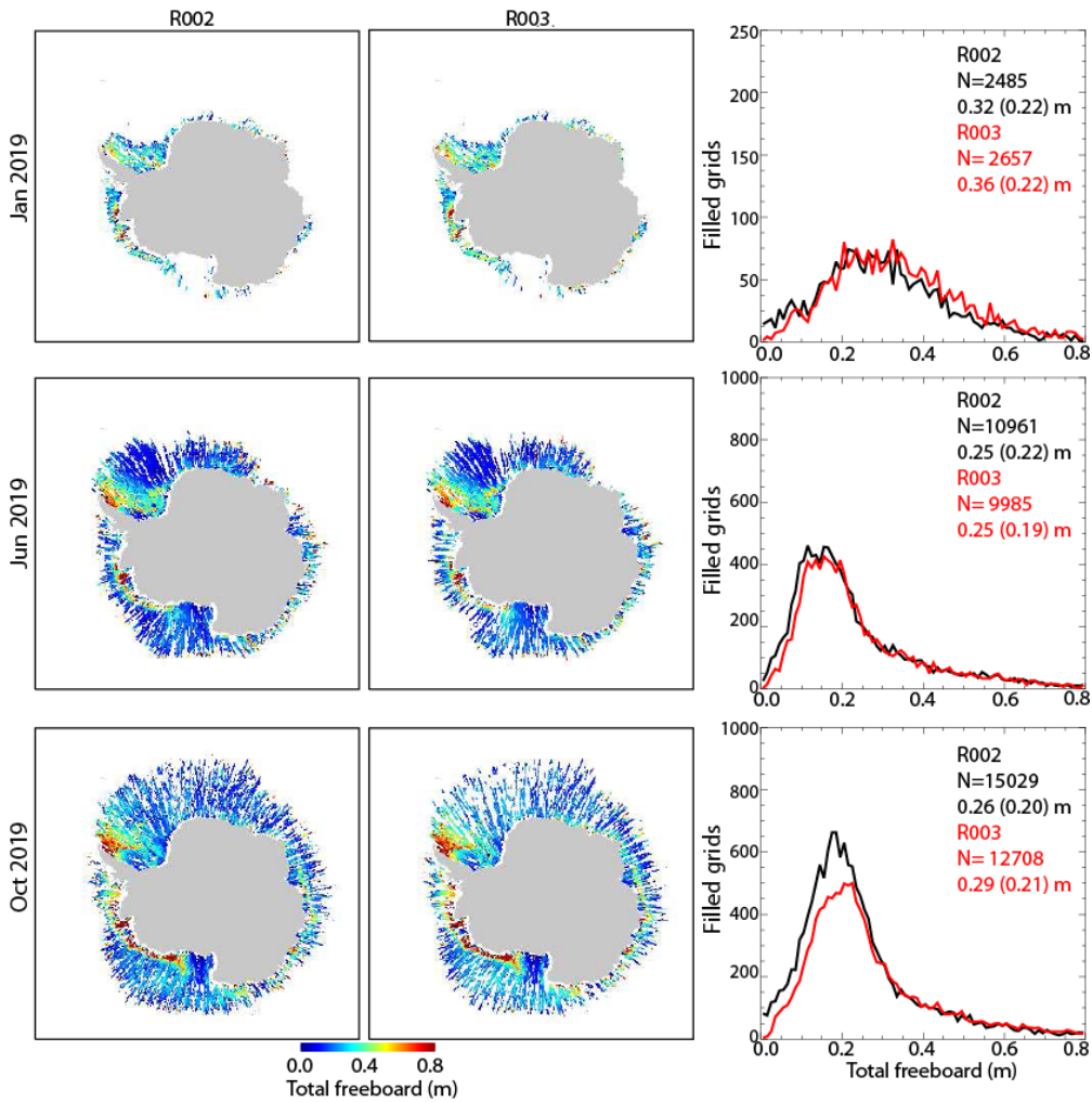
Figure 4: Same as previous figure except for the Antarctic.
