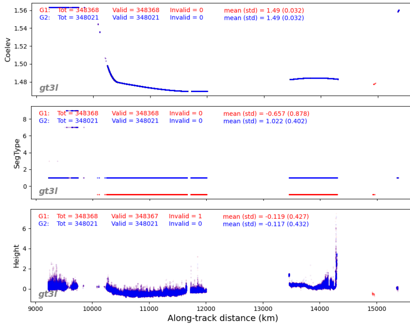
Figure 6: G1: rel005 test data, G2: rel004 data. Note the lower coelev angle after ~10000 km (in radians, top panel) indicates off-pointing in both datasets which in G1 (test rel005) triggers an invalid surface segment type (SegType = -1) with heights (bottom panel) unaffected.
