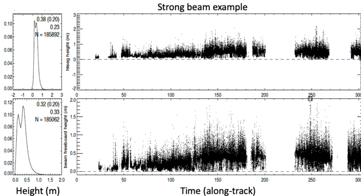
Figure 2: example ATL07 (top) and ATL10 (bottom) granule
