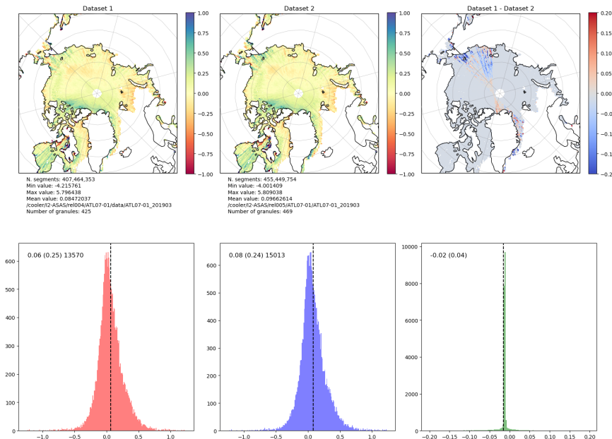
Figure 7: gridded maps (top) and histograms (bottom) of Arctic sea ice heights ( ssh\_flag = 0 ) from ATL07 during March 2019. Dataset 1: rel004, Dataset 2: test rel005. Note the difference in regions where the PODPPD flag = 4. Due to the change in along-track distance/spatial sampling during off-pointing scans it is challenging to determine any underlying bias in these data.
