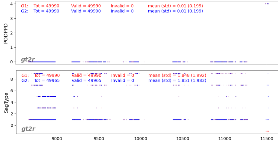
Figure 5: G1: rel005 test data, G2: rel004 data. Note the PODPPD flag of 4 in both datasets around 11500 km (top panel, right) which in the rel005/G1 test data triggers an invalid surface segment type (SegType = -1).
