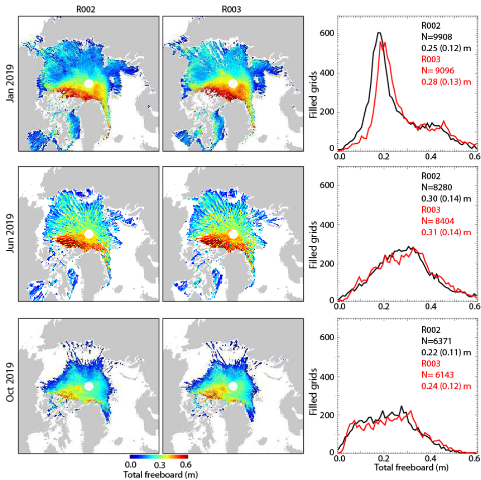
Figure 3: Changes in coverage and freeboard distributions of the Arctic Ocean sea ice cover in monthly composites of Jan, Jun, and Oct 2019. N is the number grid cells (25 by 25 km) that contains freeboard estimate. Numerical values are the mean (standard deviation) of the distributions. The distributions are not normalized and show actual population counts and provide an indication of the loss and gain of samples in each of the distribution bins.
