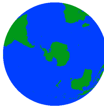
(b) Southern Hemisphere on EASE 2.0 Grid projection (Figure credited to NSIDC)
