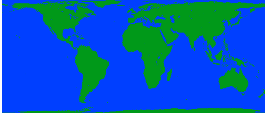
(c) Global Cylindrical EASE 2.0 Grid projection (Figure credited to NSIDC)
