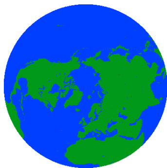
(a) Northern Hemisphere on EASE 2.0 Grid projection (Figure credited to NSIDC)
