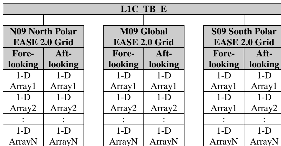
Figure 5: L1C_TB_E data organization according to projections and azimuth directions.
