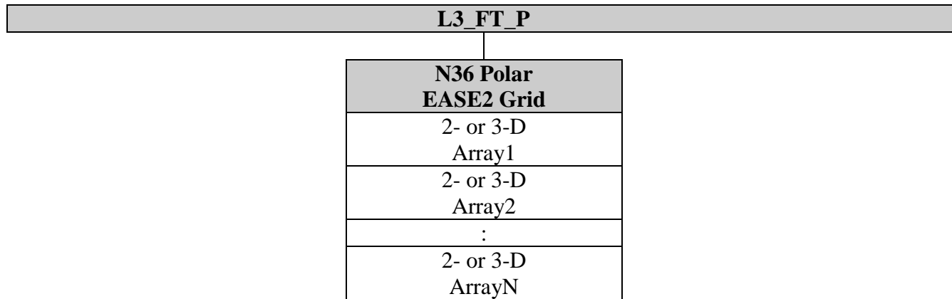
Figure 5: L3_FT_P data organization.
