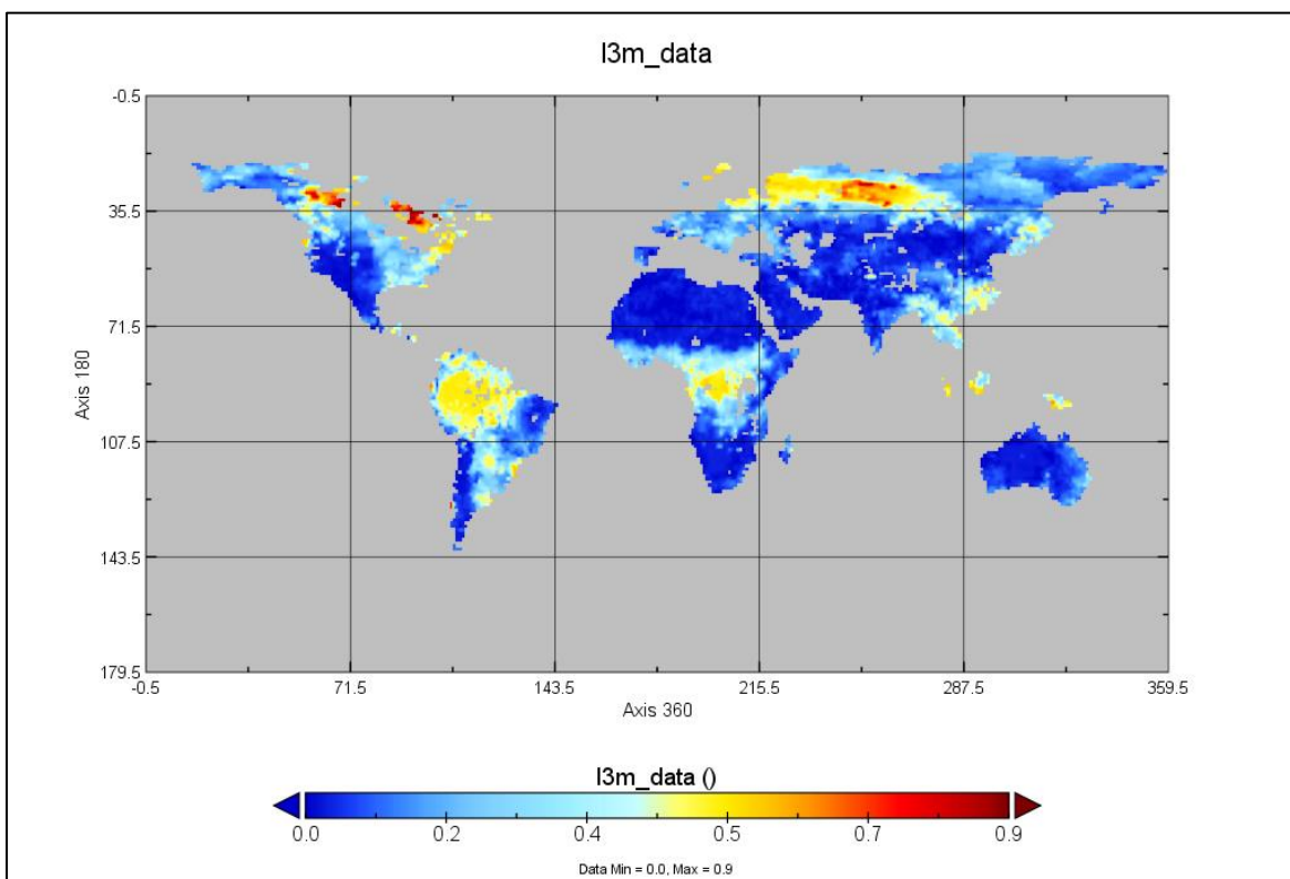
Figure 1. This plot shows Aquarius soil moisture estimates acquired using all three beams for the month of May in 2012.
