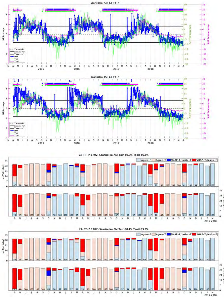
Figure 6.11. As in Figure 6.4 but for Saariselka.
