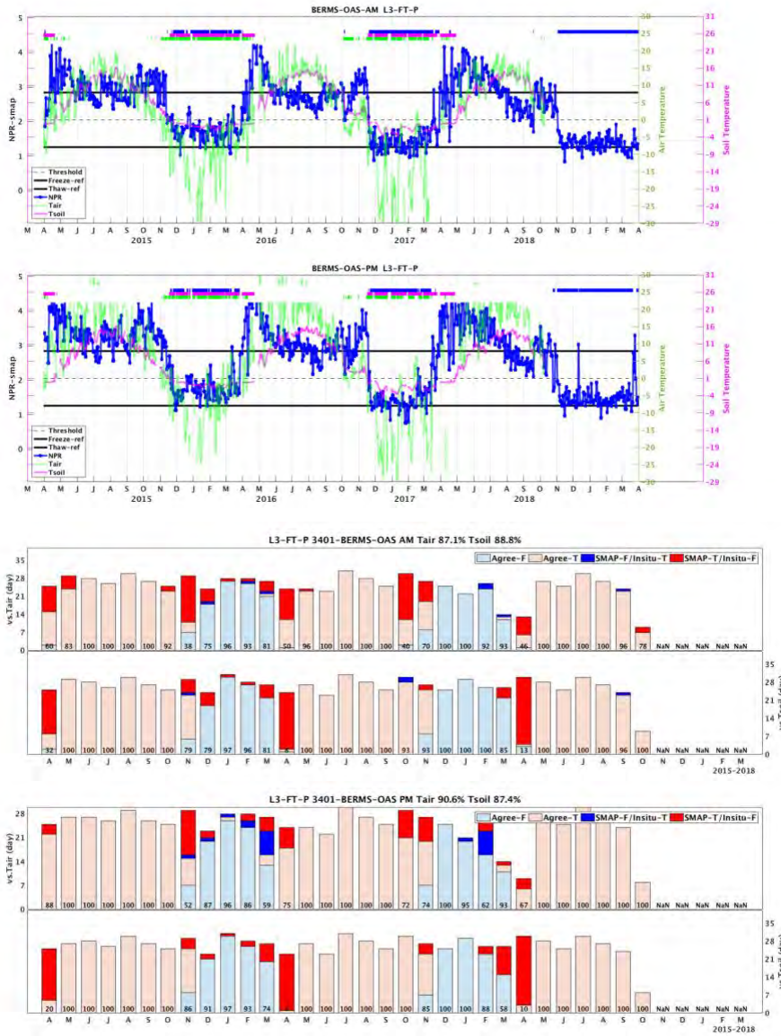
Figure 6.9. As in Figure 6.4 but for BERMS – Old Aspen.
