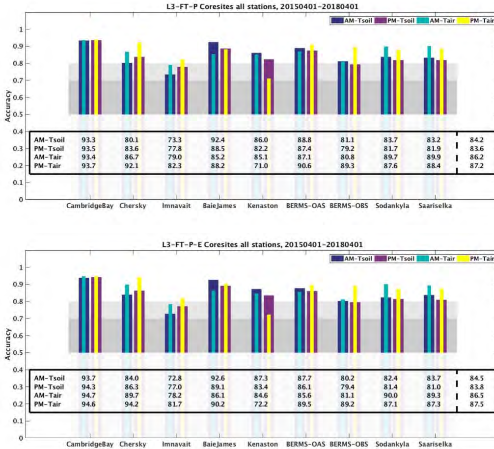
Figure 6.16. Three-year statistics for each core validation station compared with in-situ flags derived from air temperature and soil temperature with the overall statistic in the last column. Top: accuracy over standard 36km L3-FT-P; Bottom: accuracy over enhanced 9km L3-FT-P-E.
