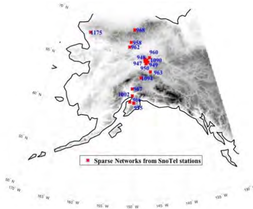
Figure 6.17. SNOTEL sites used for SMAP NPR Freeze/Thaw product evaluation.
