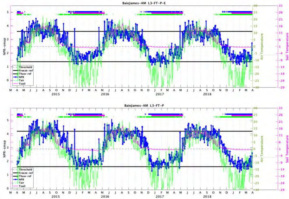
Figure 6.15. Descending overpass time series of NPR (blue line), air temperature (green line), and soil temperature (magenta) for Baie-James between L3-FT-P-E (top) and L3-FT-P (bottom). Horizontal lines on the top note the occurrence of frozen flags for SMAP derived (blue), air temperature derived (green) and soil temperature derived (magenta) conditions.
