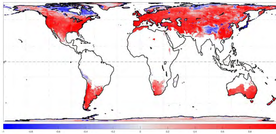
Figure 3.2. Correlation between the SMAP Tbv and GMAO surface temperature
