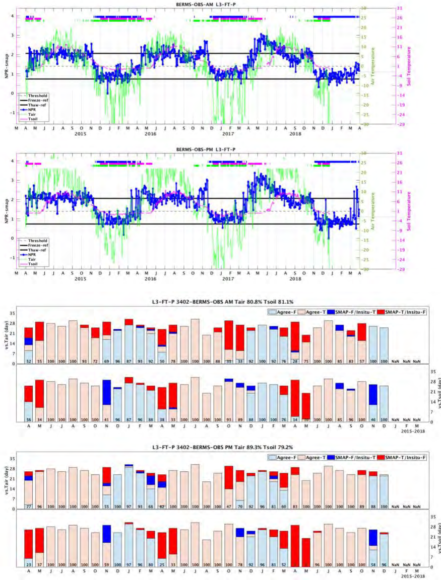
Figure 6.8. As in Figure 6.4 but for BERMS – Old Black Spruce.
