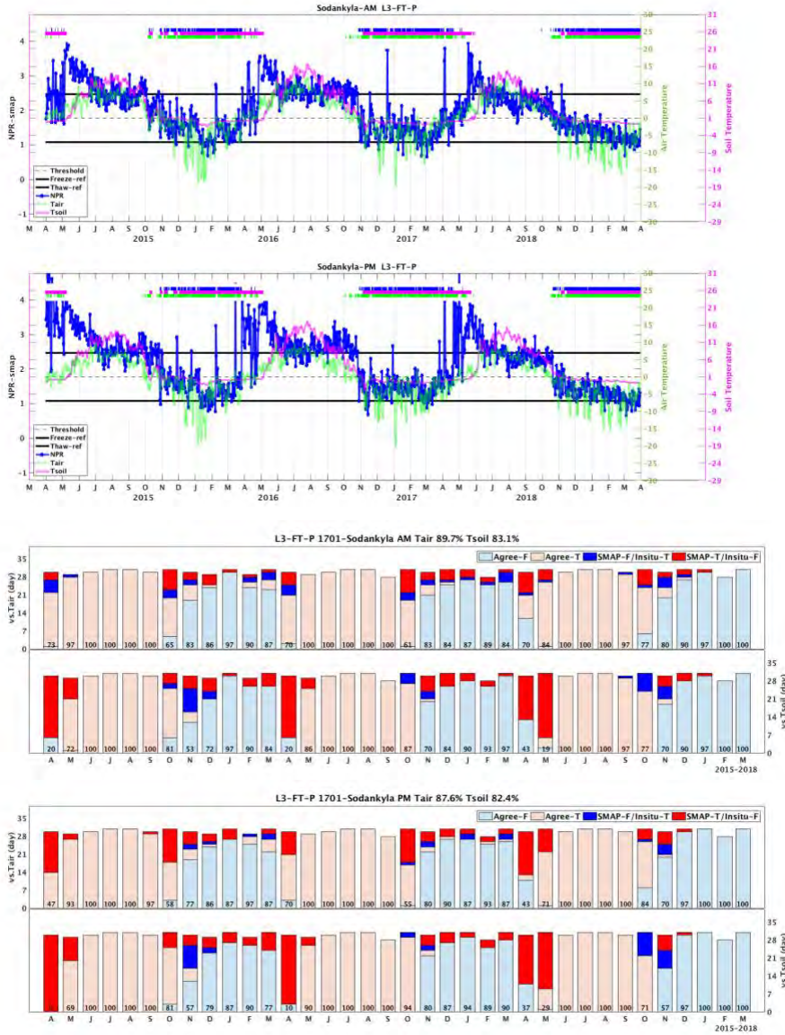
Figure 6.10. As in Figure 6.4 but for Sodankyla.
