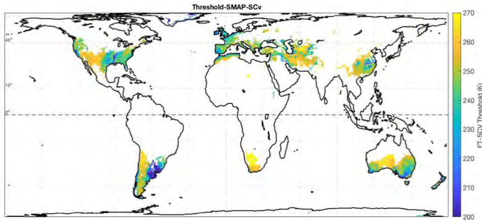
Figure 5.3. Freeze/thaw brightness temperature thresholds used for the FT-SCV extended algorithm; areas outside of the FT-SCV domain are shown in white.
