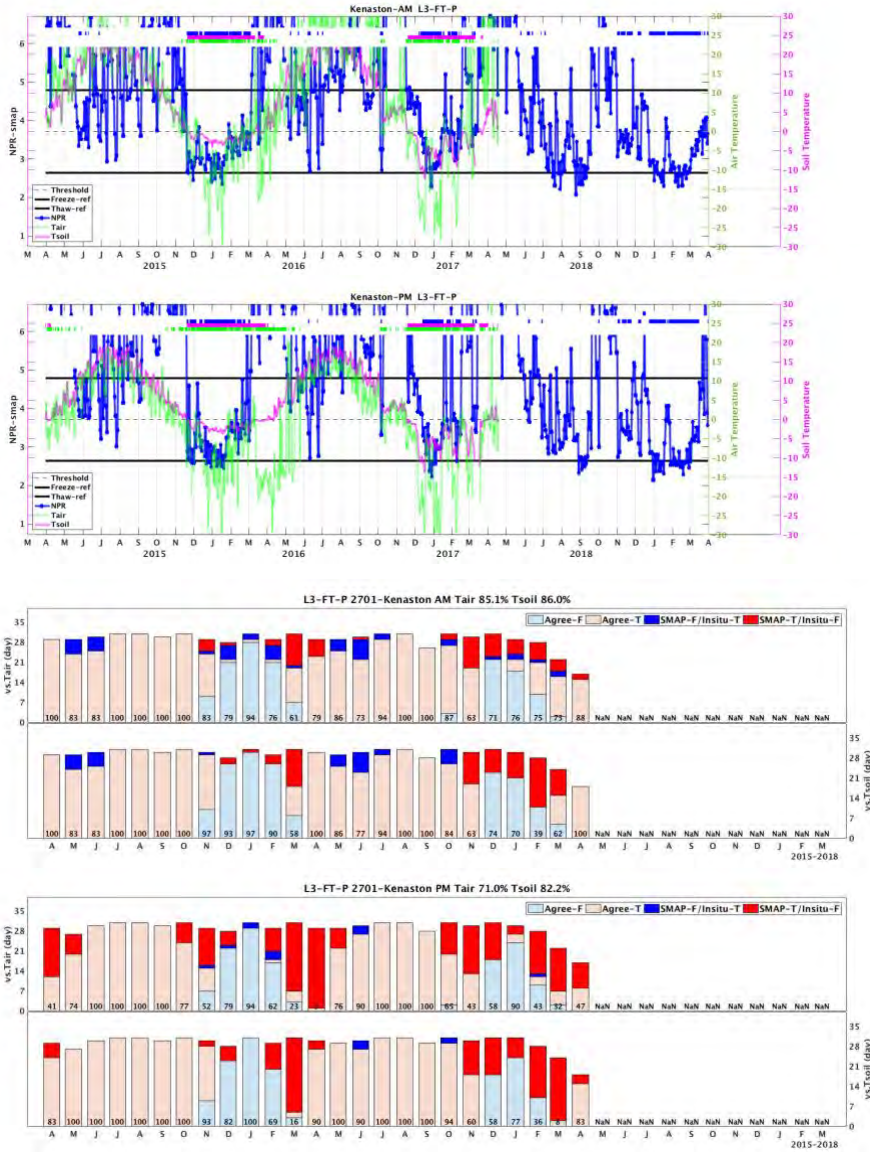
Figure 6.12. As in Figure 6.4 but for Kenaston.
