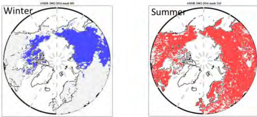
Figure 5.2. Example never thawed (Left) and never frozen (Right) masks for 1 January and 29 July.
