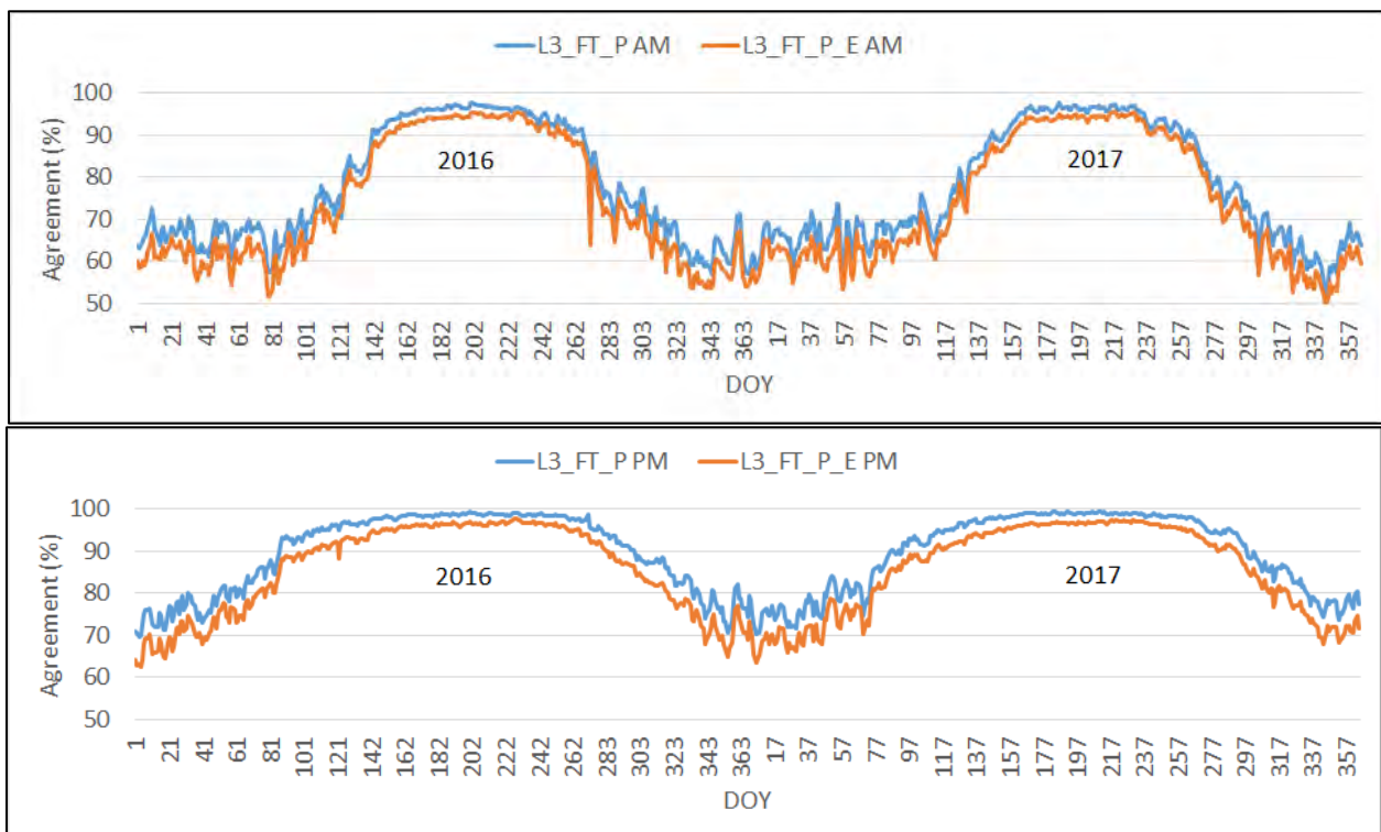
Figure 6.22. Seasonal pattern of SMAP daily mean FT classification agreement (%) in relation to WMO in-situ surface air temperature measurements for AM (top) and PM (bottom) overpass results; blue and red lines denote respective 36-km and 9-km grid results.
