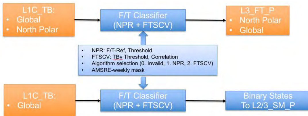
Figure 3.1. Processing sequence for generation of the L3_FT_P product and the binary freeze/thaw state flag for use in L2_SM_P.
