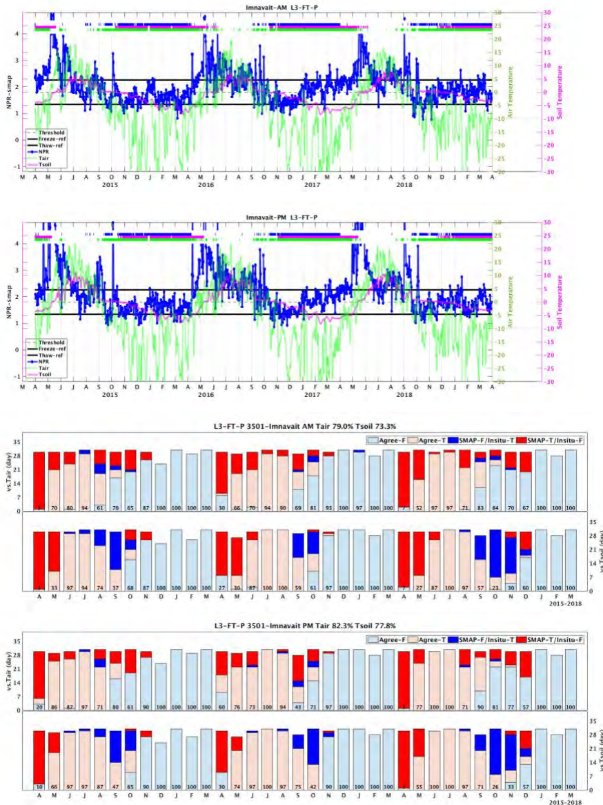
Figure 6.5. As in Figure 6.4 but for Imnavait, AK.
