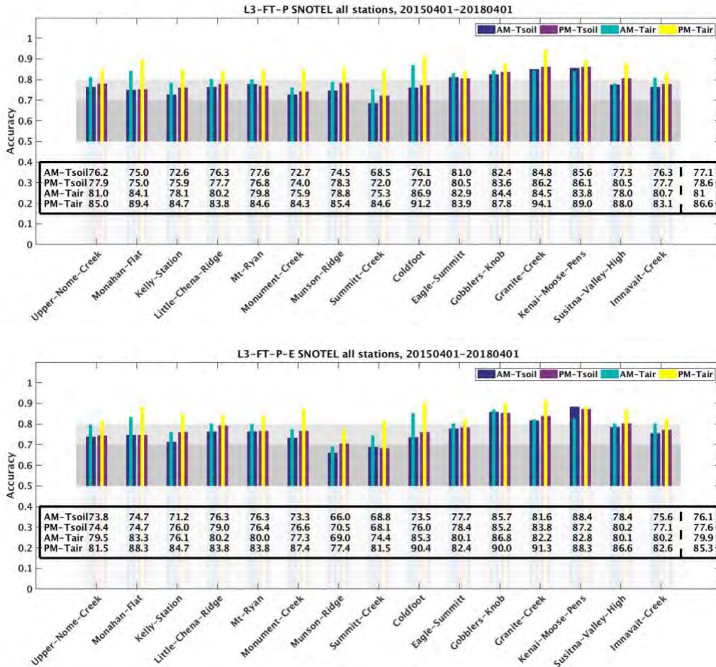
Figure 6.19. Summary of SMAP NPR FT three-year accuracy over each SNOTEL validation site for both ascending and descending pass results. The overall statistic is in the last column.
