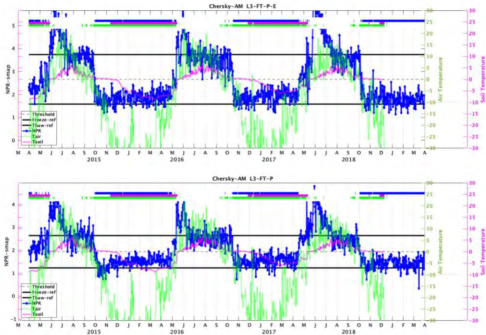
Figure 6.14. Descending overpass time series of NPR (blue line), air temperature (green line), and soil temperature (magenta) for Chersky between L3-FT-P-E (top) and L3-FT-P (bottom). Horizontal lines on the top note the occurrence of frozen flags for SMAP derived (blue), air temperature derived (green) and soil temperature derived (magenta) conditions.
