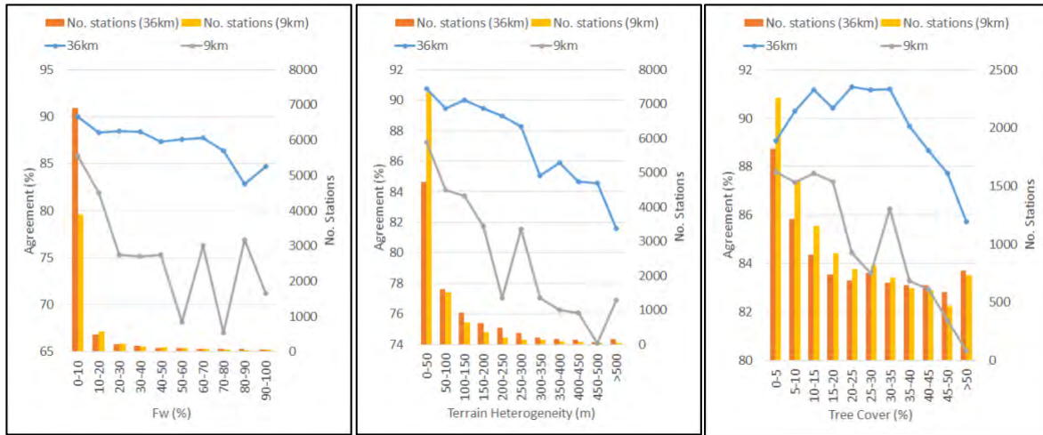
Figure 6.24. Dominant spatial heterogeneity indicators affecting 2016-2017 PM overpass FT classification agreement for individual grid cells, including open water fraction (Fw), terrain heterogeneity, and percent tree cover.
