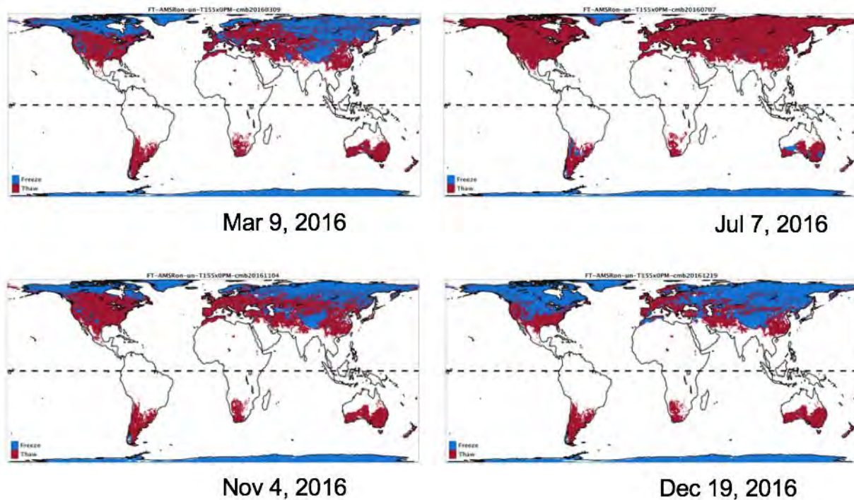
Figure 6.1 Snapshot FT map over 2016 for selected days in spring, summer, fall and winter.
