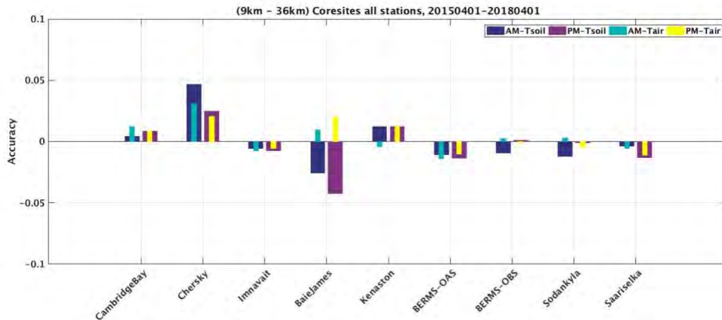
Figure 6.13. Difference in FT flag agreement, L3_FT_P_E minus L3_FT_P for descending and ascending overpasses. Positive values correspond to improved agreement for the enhanced resolution product; negative values correspond to degraded agreement.
