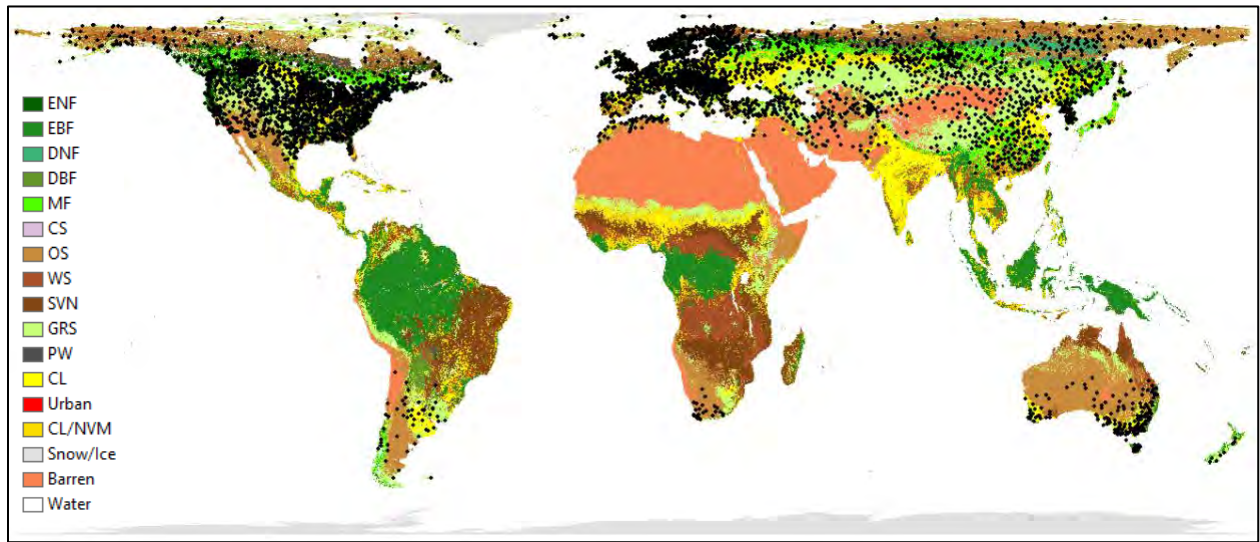
Figure 6.21. MODIS MCD12Q1 IGBP Land cover map showing WMO weather stations (black dots) used for SMAP FT validation assessment over the global domain.
