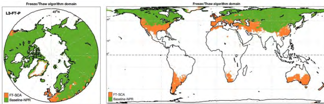
Figure 3.3. Freeze/thaw algorithm Polar domain (Left) and Global domain (Right) showing areas where FT-SCA and NPR algorithms are applied.
