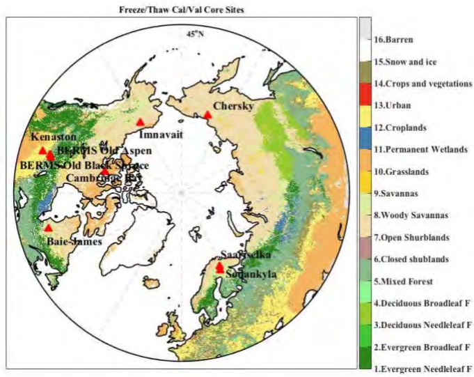
Figure 6.2. Core sites used for Freeze/Thaw validation.
