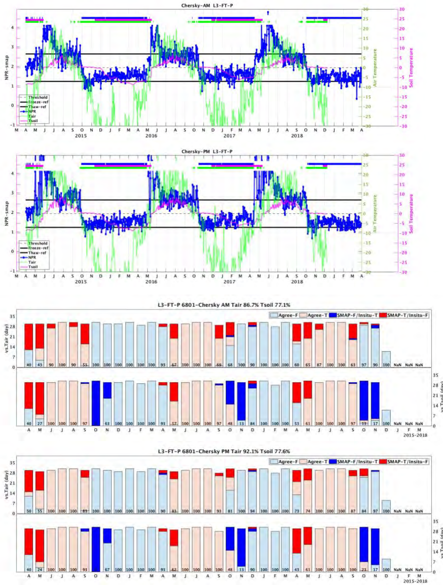
Figure 6.6. As in Figure 6.4 but for Chersky.
