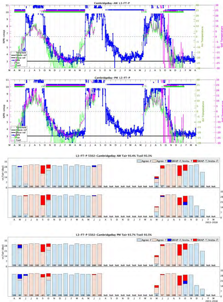
Figure 6.4. (a) Descending (AM) and (b) ascending (PM) overpass time series of NPR (blue), air temperature (green), and soil temperature (magenta) for Cambridge Bay. Horizontal lines on the top note the occurrence of frozen flags for SMAP derived (blue), air temperature derived (green) and soil temperature derived (magenta) conditions. (c) AM Monthly summary of freeze/thaw flag agreement and error. The bars show the agreement and error days. The number in the bottom of each bar is the accuracy in percentage for each month.
