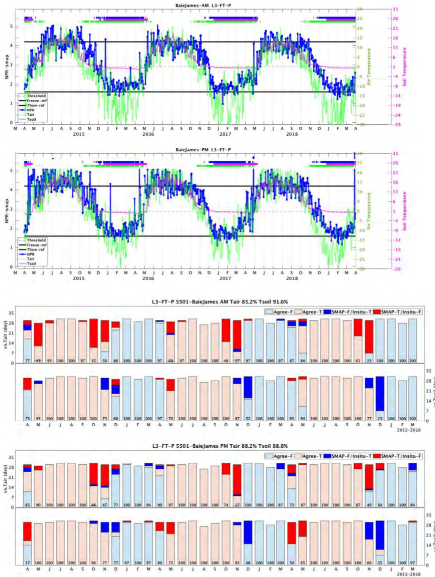
Figure 6.7. As in Figure 6.4 but for Baie-James.
