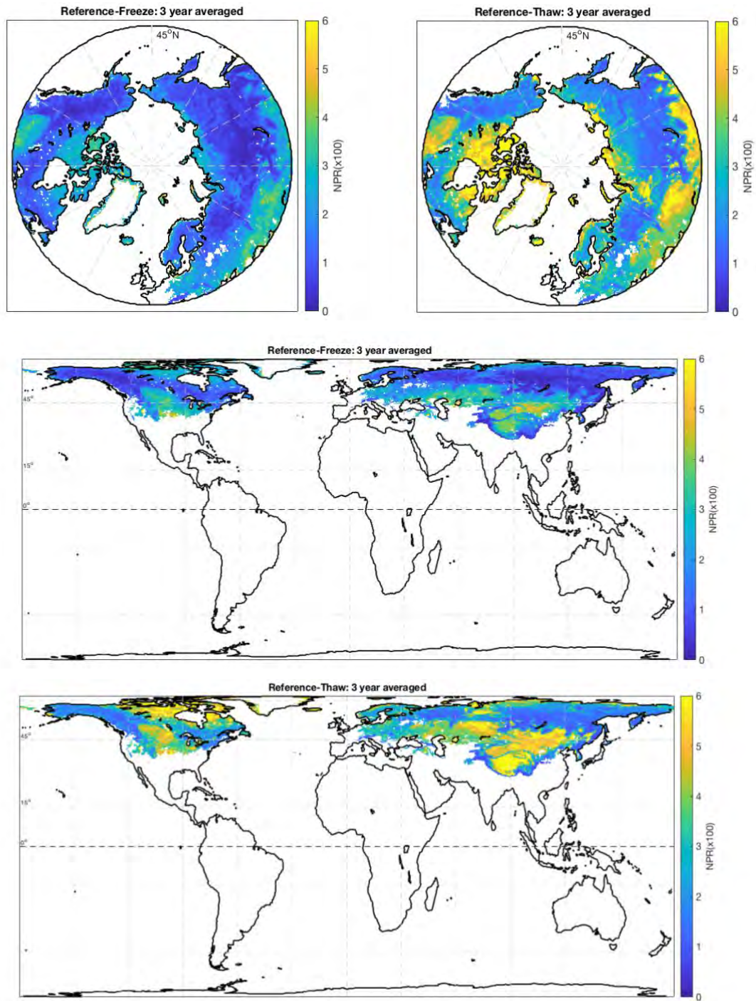
Figure 5.1. SMAP NPR algorithm (a) freeze and (b) thaw references in polar grid; NPR (c) freeze and (d) thaw references in global grid. Units are NPR scaled by 100 and averaged over three years (2015-2018).
