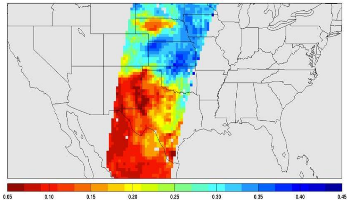
Figure 11. Example of SMAP retrieved soil moisture in cm 3 /cm 3 . The half-orbit swath pattern is simulated using the orbital sampling module on the SMAP Algorithm Development Testbed.
