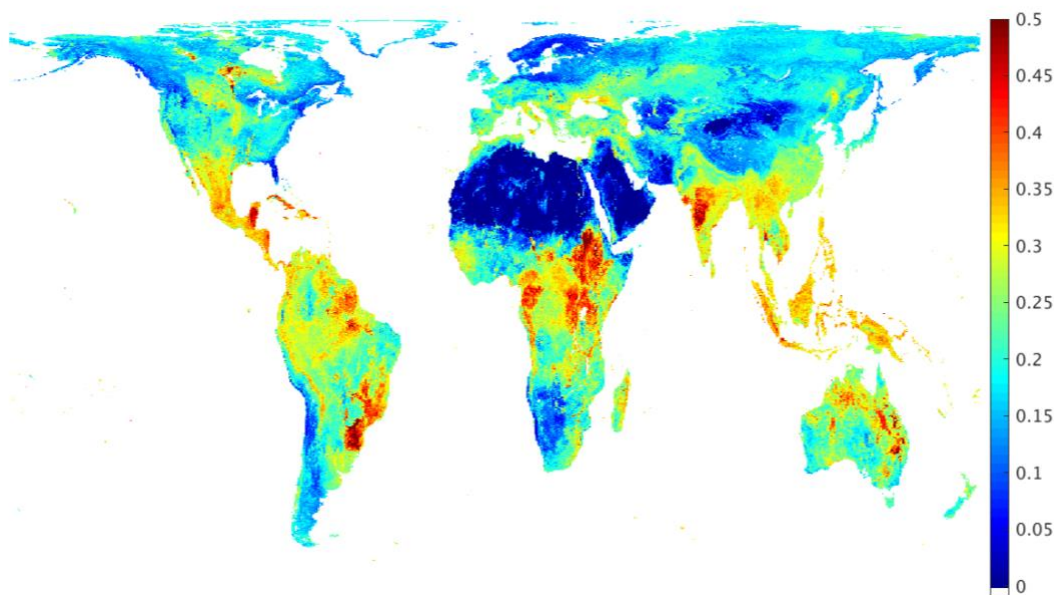
Figure 27. Global clay fraction from SoilGrid250m soil texture database (available at https://openlandmap.org ).
