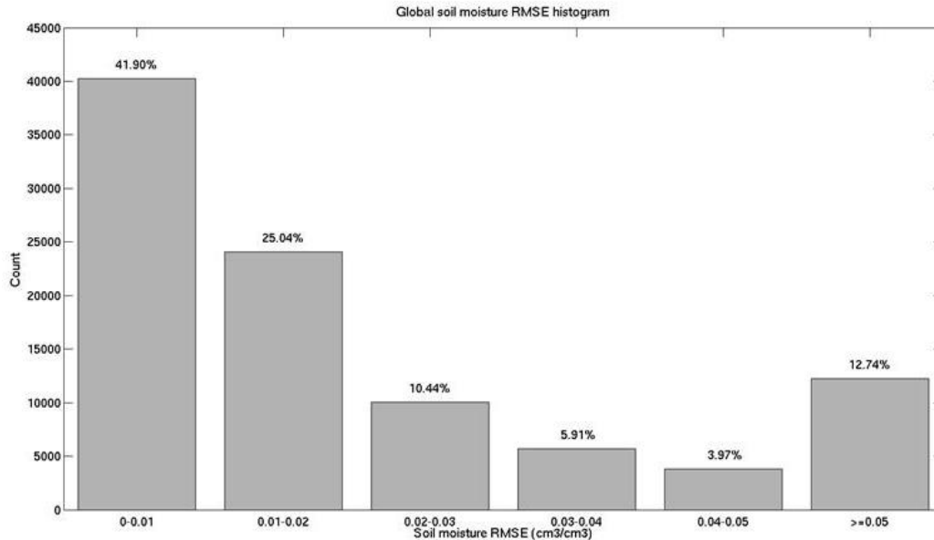
Figure 22b. Histogram of global soil moisture retrieval error based on simulation shown in (a). Approximately 83% of the area in the SMAP land mask has a soil moisture retrieval error \leq 0.04 cm 3 /cm 3 .
