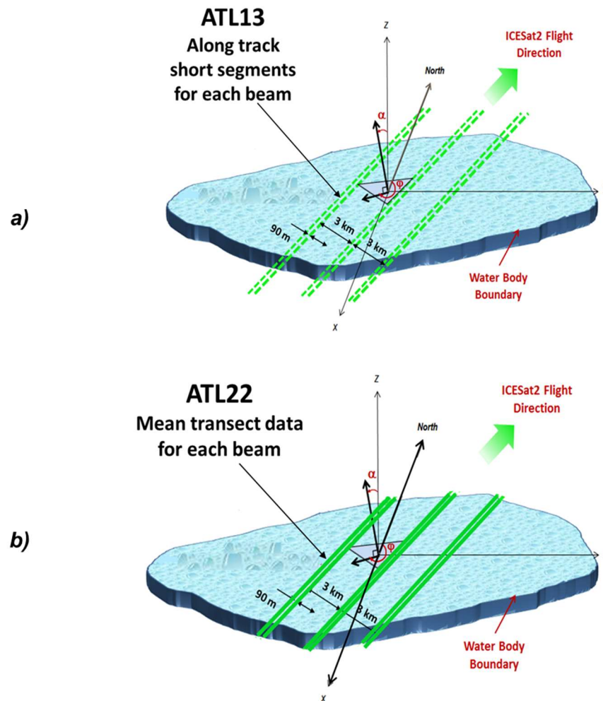
Figure 1-1 a) Schematic of principal ATL13 Inland Surface Water along track data products includes surface height statistics, subsurface attenuation, significant wave height (SWH) and coarse bottom topography. Height statistics are reported for variable segment lengths of 100 signal photons. Estimated accuracy is 5-8 cm per 100 signal photons. b) Comparison schematic of principal ATL22 Release 2 Mean Inland Surface Water data products to be available in July 2021.
