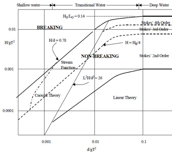
Figure 2-3 Parameter space for wave theories based on normalized height ( H/g\tau^2 ) and water depth ( d/g\tau^2 ), where g is gravity constant, and \tau is wave period, after Le Méhauté, B. (1976).
