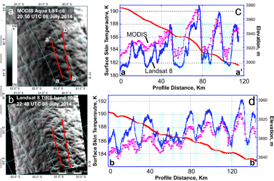
Figure 3. Comparison of mid-winter Aqua MODIS LST c6 (a) and Landsat 8 TIRS band 10 (b) image data adjusted to match MODIS LST regionally, under clear sky and low temperature conditions; c and d, MODIS LST (pink line) and Landsat 8 TIRS (blue line) temperatures and elevation (red line) profiles (a-a' and b-b' in image panels; elevation for a-a' from Bamber et al., 2009; for b-b', Bell et al., 2011). Light blue shaded regions mark areas of flat or reverse slope.
