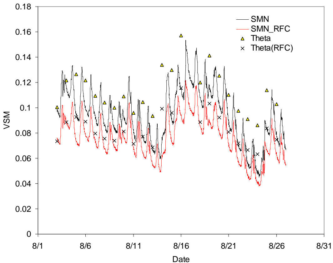
Figure 1: Time series of soil moisture network and rock corrected soil moisture network and the dielectric average and rock fraction corrected dielectric average.
