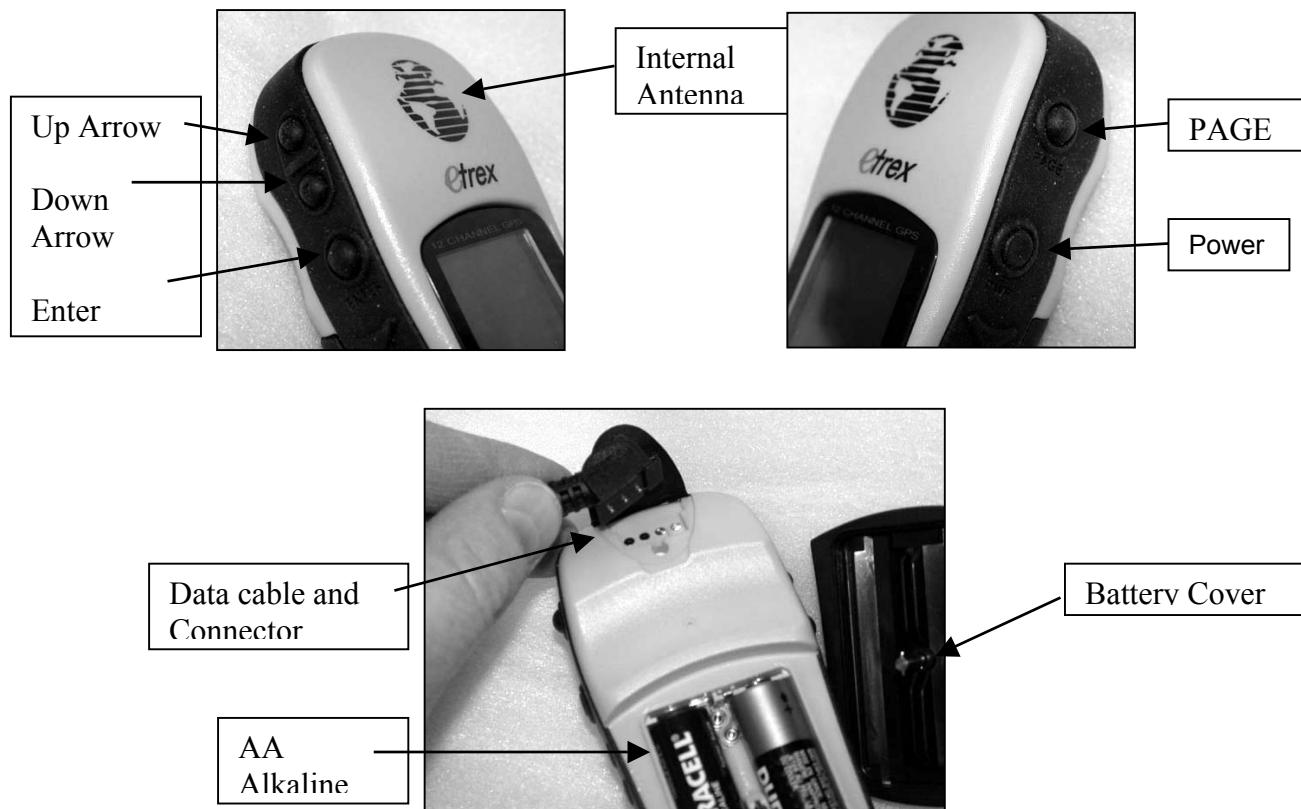
Figure 61. GPS features.
