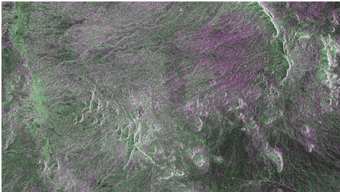
Figure 28. ASAR image of the Walnut Gulch Watershed on September 9, 2003. VV was assigned purple and VH green.
