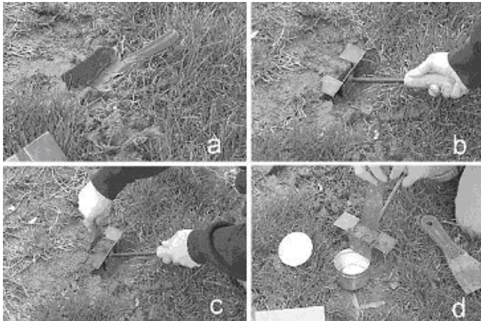
Figure 48. How to take a gravimetric soil moisture sample.
