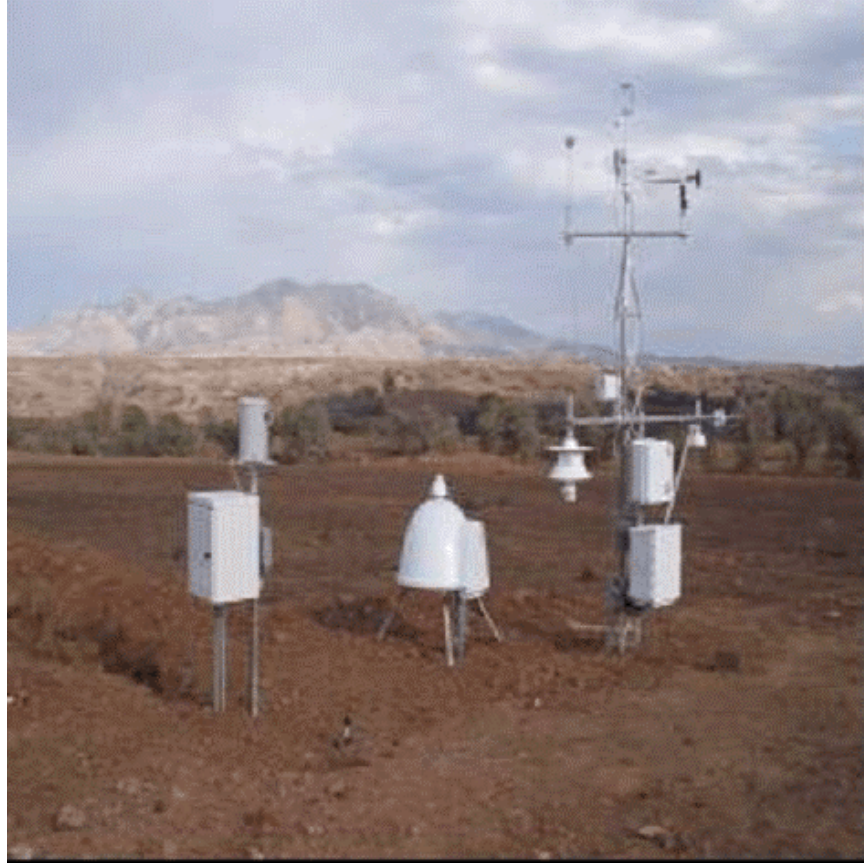
Figure 41. Audubon Research Ranch surface flux tower.
