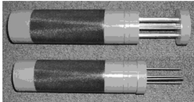
Figure 46: SMITY, Soil Moisture Insertion Tool, with slider extended and retracted.
