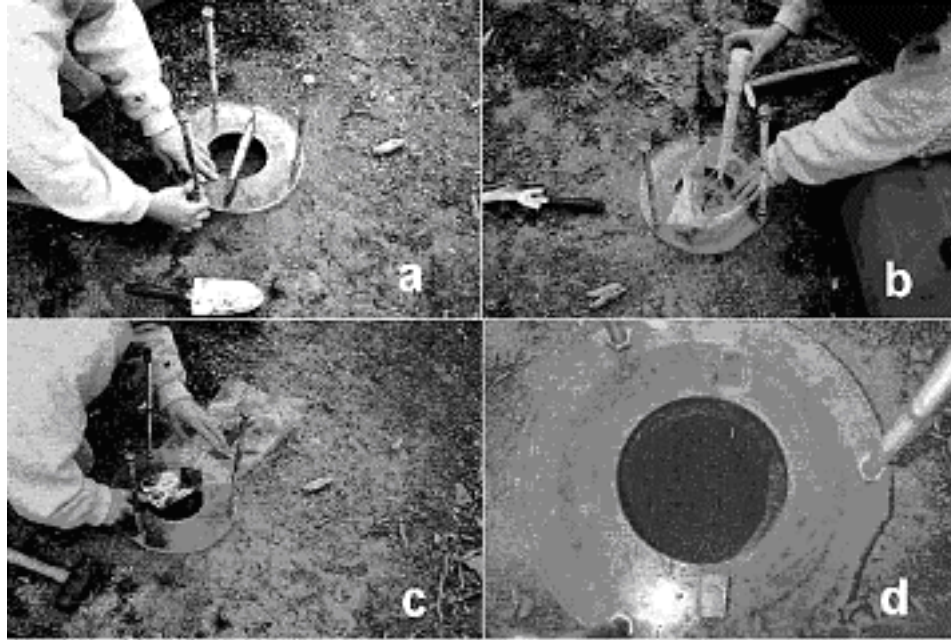
Figure 50. How to take a bulk density sample
