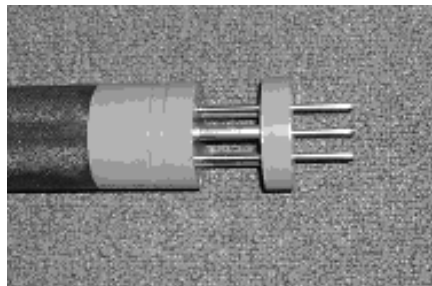
Figure 47: Close-up of the SMITY slider.
