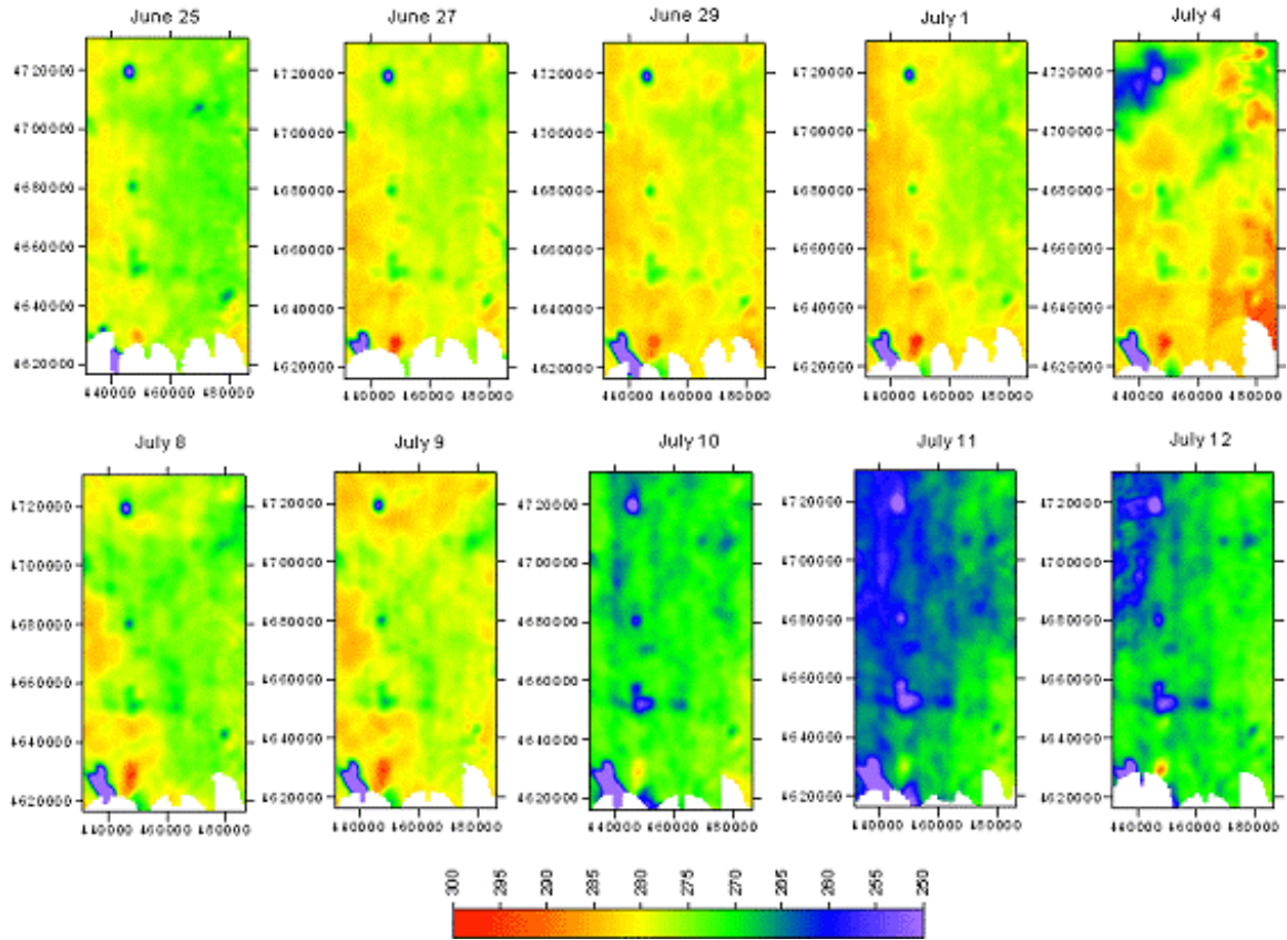
Figure 24. PSR C-band (7.32 GHz) horizontal polarization brightness temperature observations over the SMEX02 region.
