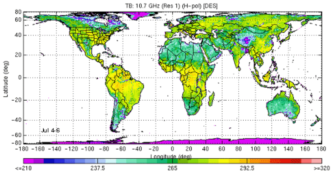
Figure 27. Example of AMSR-E brightness temperature image, three-day global composite.
