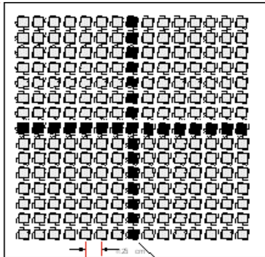
Figure 25. Antenna patch array shown configured for measuring using a cross “+” configuration.
