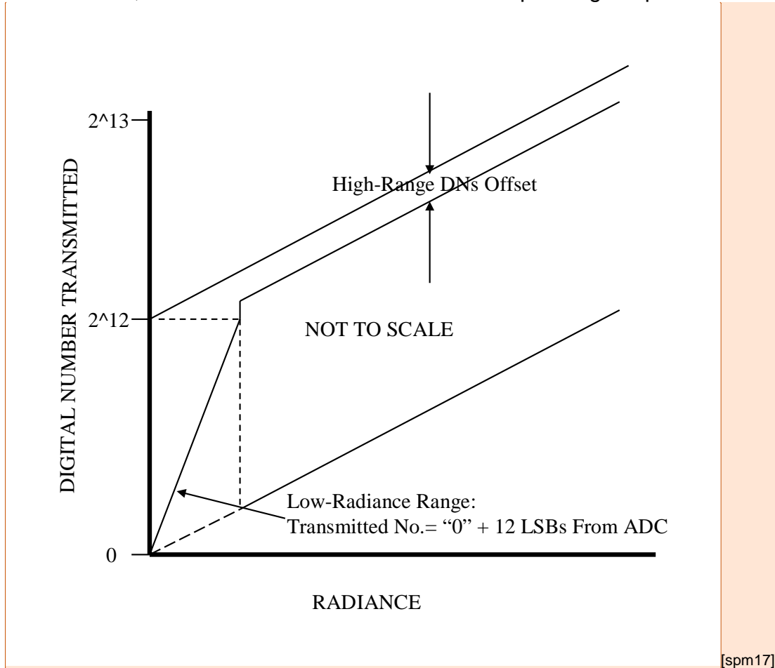
Figure 12: VIIRS Dual Gain 'M' Band Gain Switching
