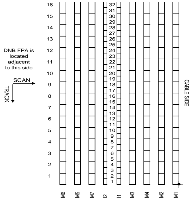
Figure 10: VIIRS Vis/NIR Detector Lay-out [spm14]
