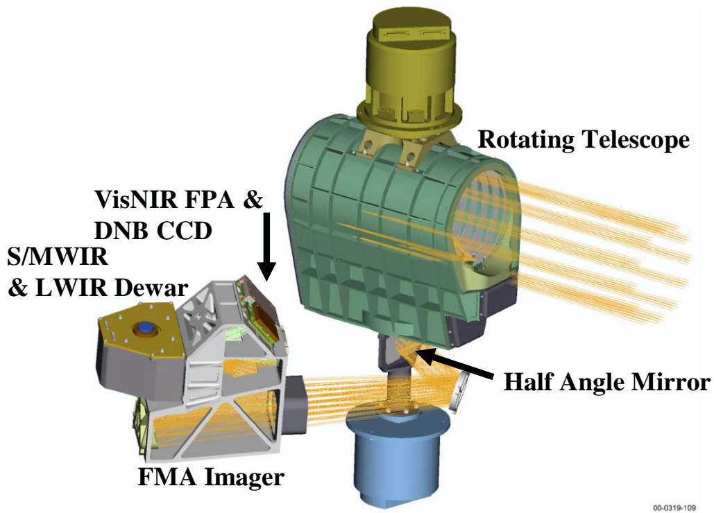
[spm11] Figure 8: VIIRS Optical Path
