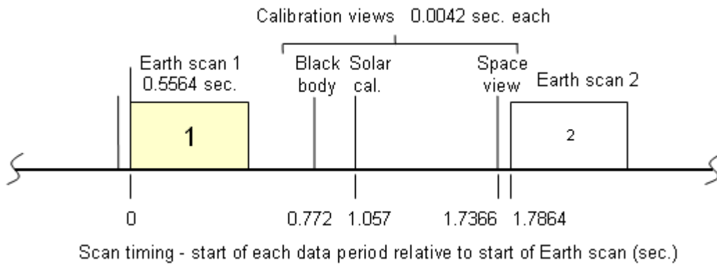
Figure 7: Timeline of Typical VIIRS Scan [spm10]
