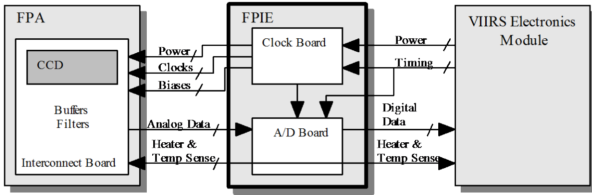
Figure 13: Simplified VIIRS DNB Block Diagram [spm18]
