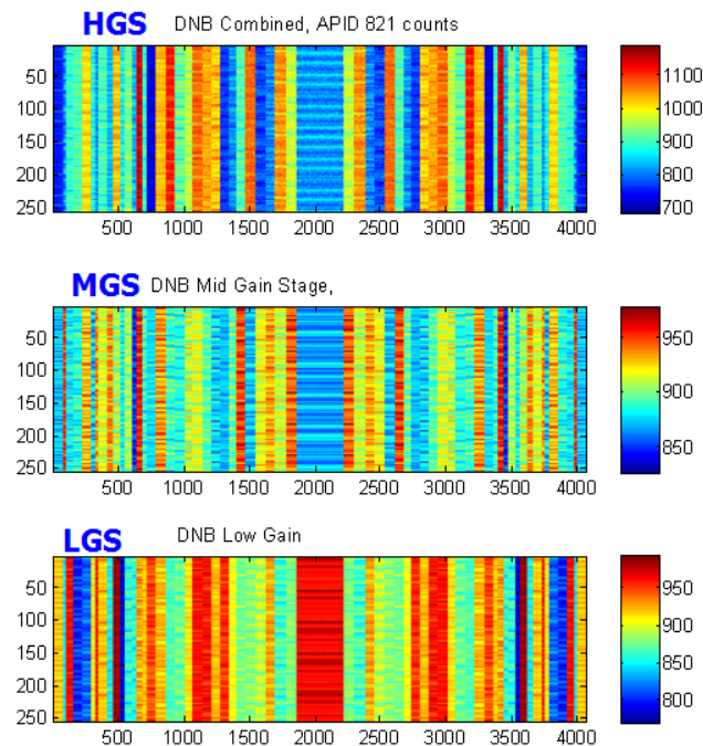
Figure 24: Simulated raw counts for 16 scans of dark earthview data for LGS, MGS and HGS
