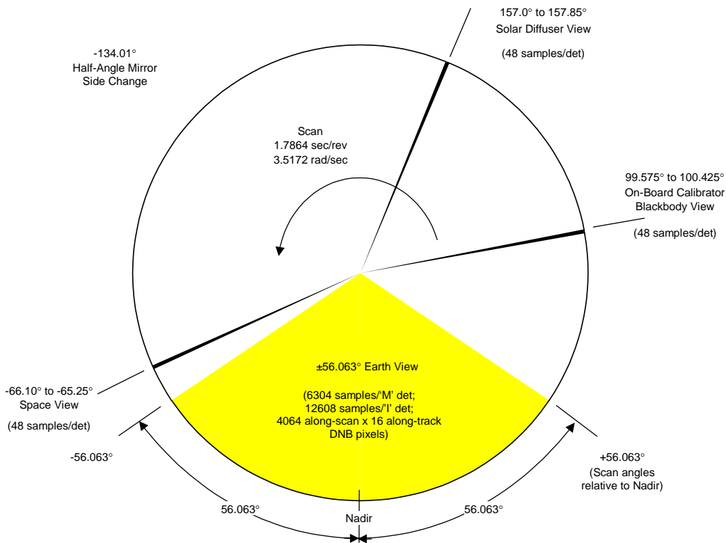
Figure 6: Diagram of VIIRS Scan Pattern [GJM9]
