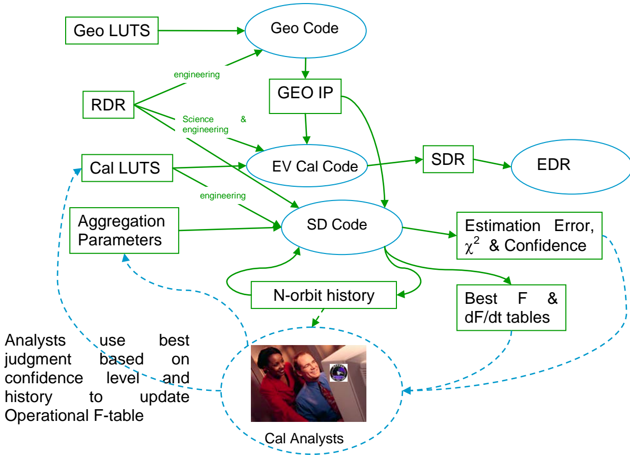
Figure 38: Flow diagram of SD Multi-orbit history and aggregation.
