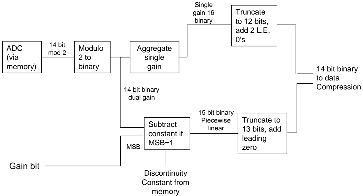
Figure 17: VIIRS 'M' and 'I' Band Data Representation [spm28]
