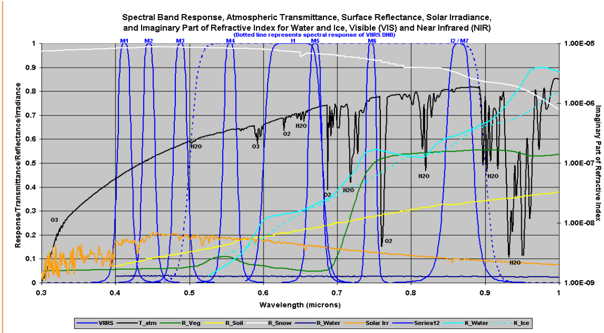
Figure 1: VIIRS Spectral Bands; Visible and Near Infrared
