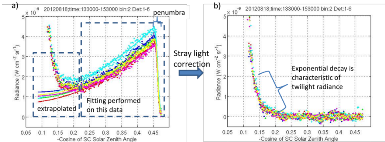
Figure 32: a) Fitting of Earth view data to create stray light offset. Data are shown as dots and fits are shown as solid lines. Only data for detectors 1-6 are shown in the figure. b) Radiance corrected for stray light.
