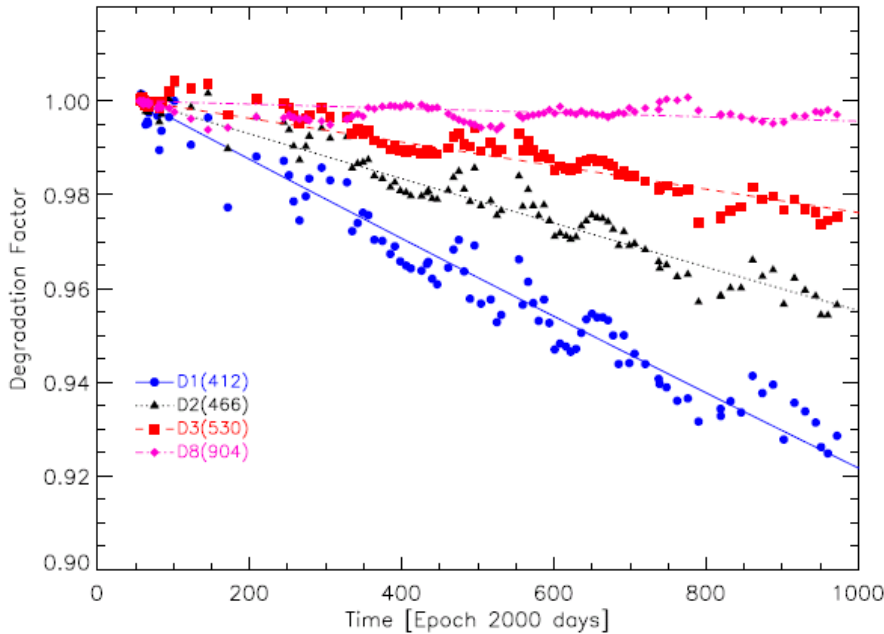
Figure 22: Changes to MODIS Terra SD reflectance trended over a 1000 days.
