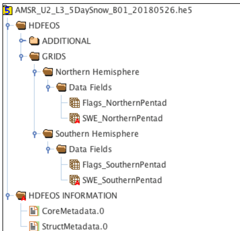
Figure 1. Fields included in this data set as displayed with HDFView software.
