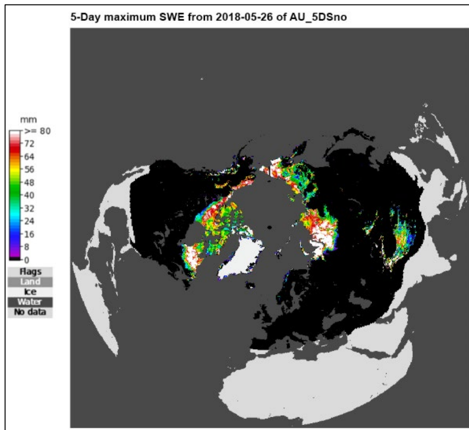
Figure 2. AMSR2 Northern Hemisphere 25 km 5-Day SWE from 2018-05-26.
