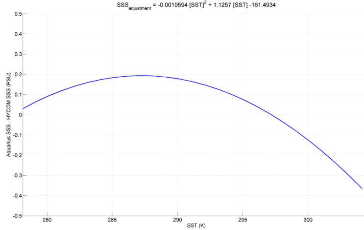
Figure 6: Functional form of the adjustment for dependence on SST. In the derivation of equation (16) cold water T_S < 5^\circ C has been excluded. However, the adjustment seems to also work in cold water and seems to work down to T_S = 0^\circ C . Therefore equation (16) is used for all SST.
