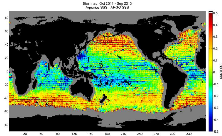
Figure 5: Mean SSS bias for Oct 2011 to Sep 2013 for the Aquarius standard SSS compared to gridded ADPRC (University of Hawaii) ARGO salinity. The data are resampled to one-degree, monthly map. The monthly SSS difference is then averaged over the two-year time period.
