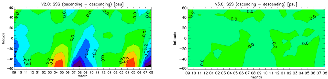
Figure 3: Hovmoeller plot of the monthly salinity difference between ascending and descending Aquarius swaths. The x-axis is time (months since September 2011) and the y-axis is latitude. Left panel: Using the geometric optics (GO) model for calculating the reflected galactic radiation (V2.0). Right panel: After adding the empirical symmetrization correction (V3.0).
