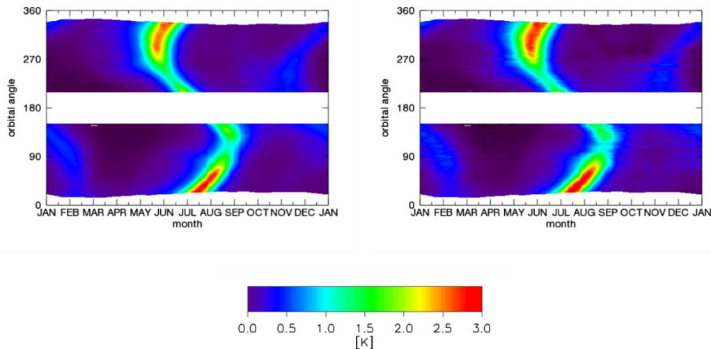
Figure 4: TA galactic reflected (average of V and H pol) for Aquarius horn 3. Left: GO (V2.0), right: after adding the empirical correction (V3.0). The x-axis is time of the sidereal year. The y-axis is the orbital position angle (z-angle).
