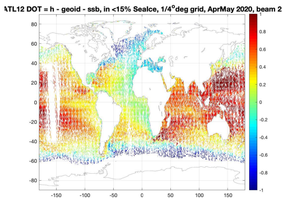
Figure 6. ATL12_20200401021904_00850701_003_01.h5 to ATL12_20200513123852_07330701_003_01.h5 DOT averaged in 1/4^\circ bins for sea ice concentration <15\% .
